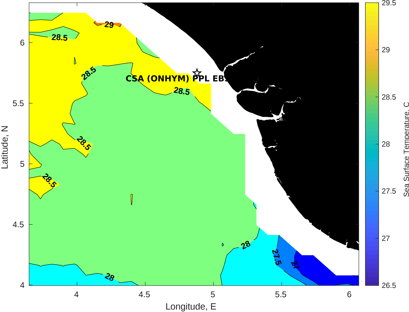
SST for CSA (ONHYM) PPL EBS - Nigeria at 08-Nov-2025 00:00:00
