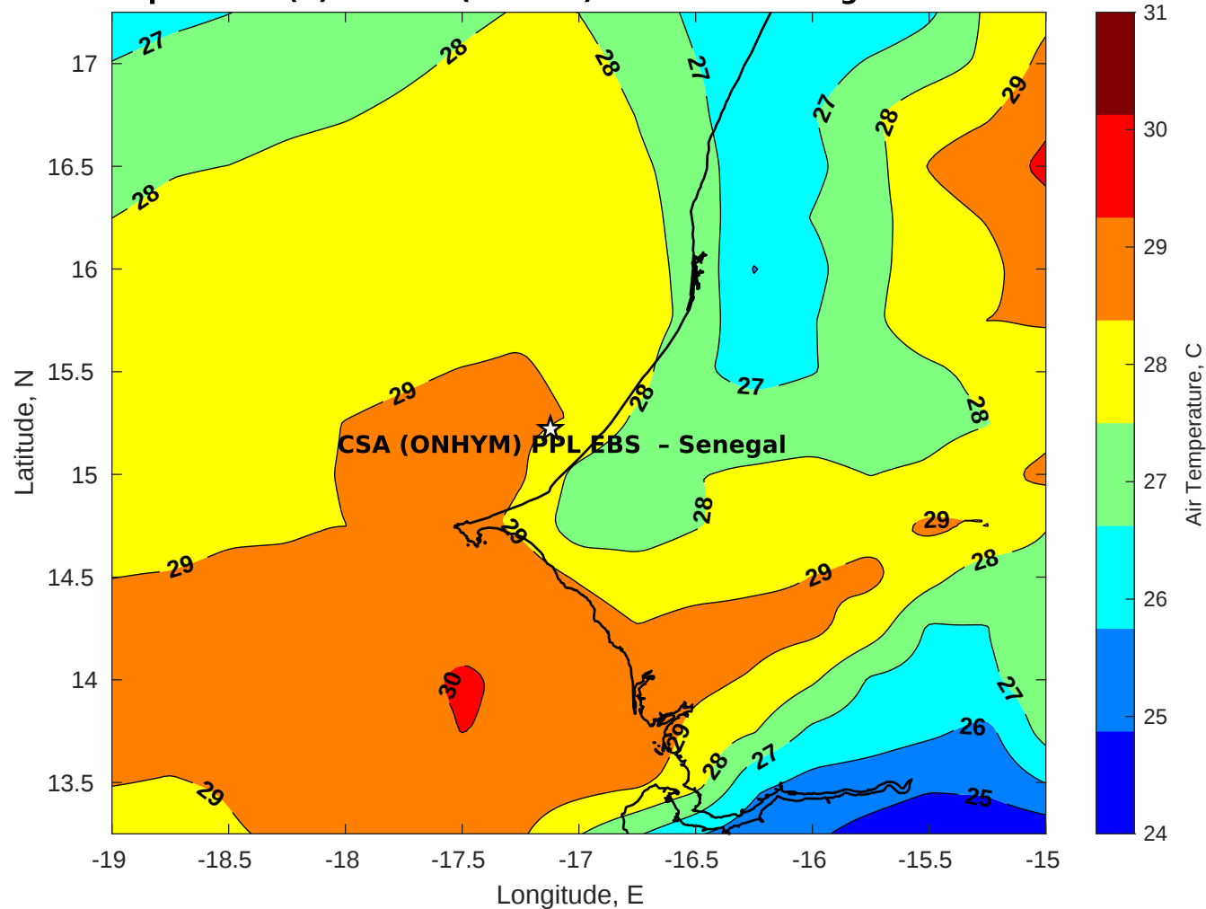
Air Temperature (C) for CSA (ONHYM) PPL EBS - Senegal at 09-Nov-2025
