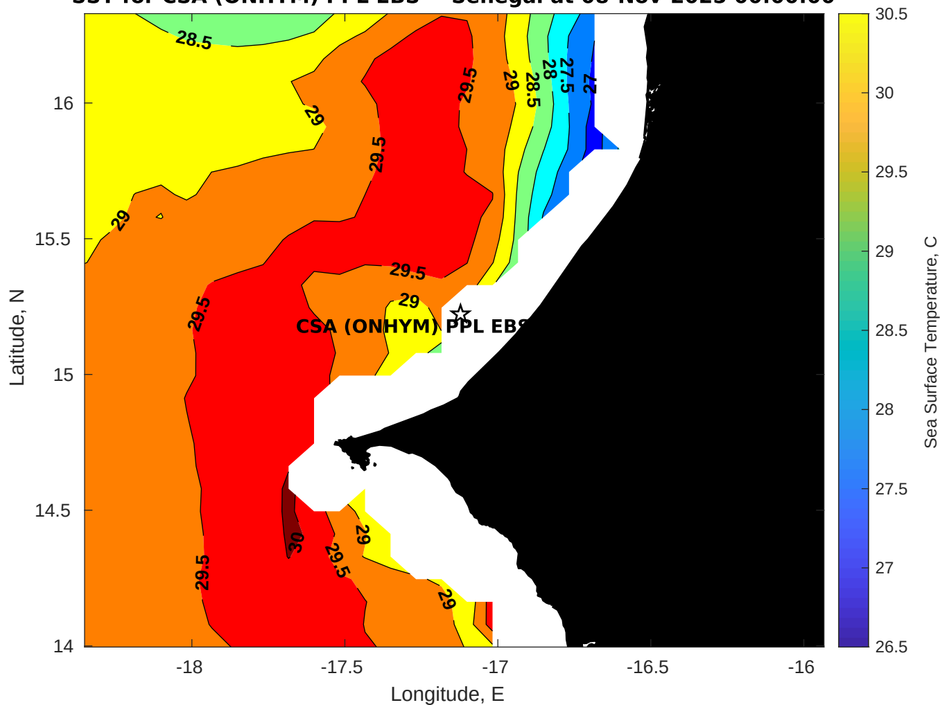
SST for CSA (ONHYM) PPL EBS - Senegal at 08-Nov-2025 00:00:00
