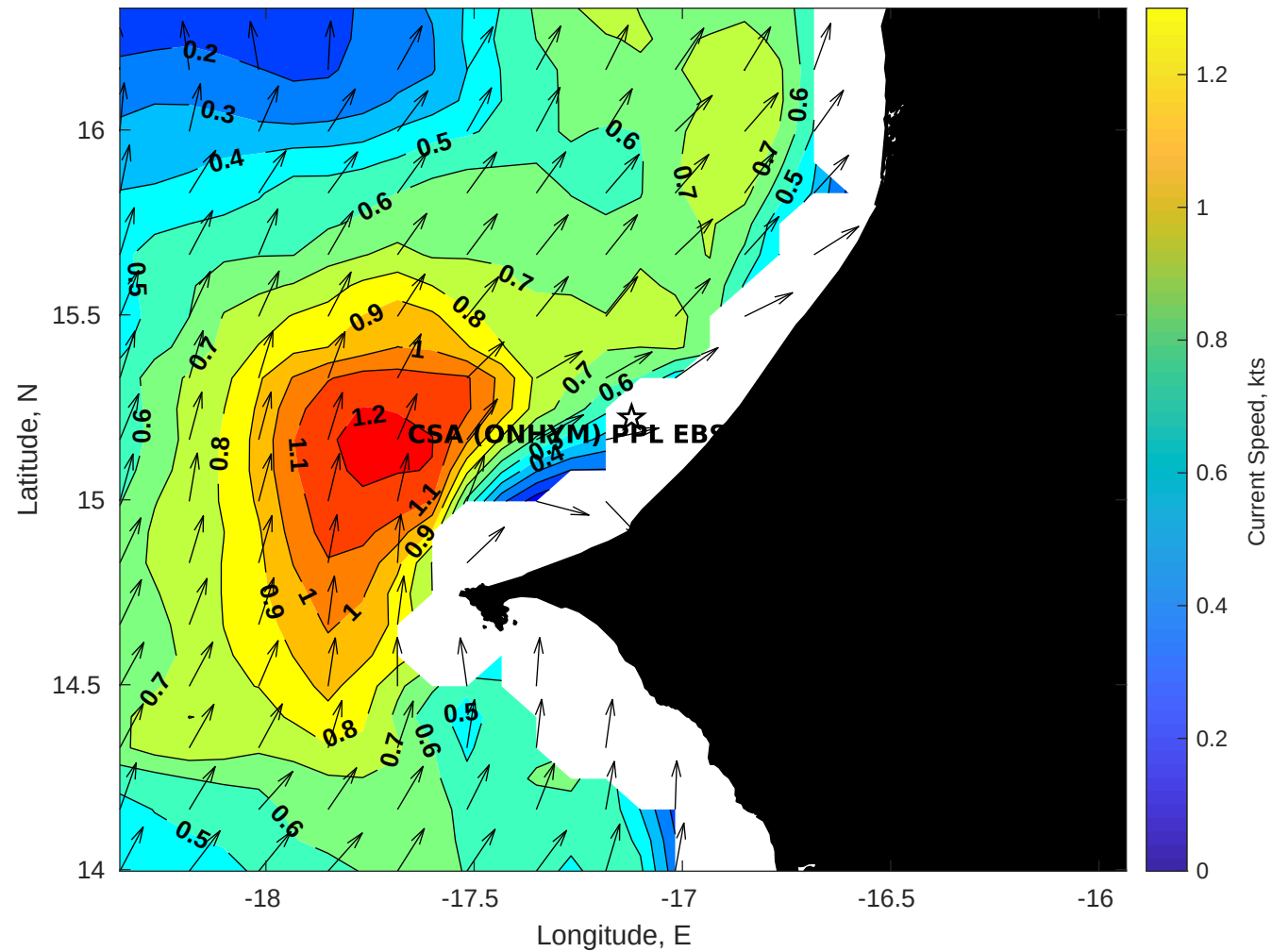
Surface Currents for CSA (ONHYM) PPL EBS - Senegal at 08-Nov-2025 00:00:00
