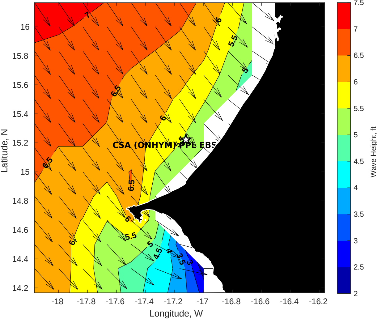
Wave Height (ft) for CSA (ONHYM) PPL EBS - Senegal at 09-Nov-2025 09:00:00
