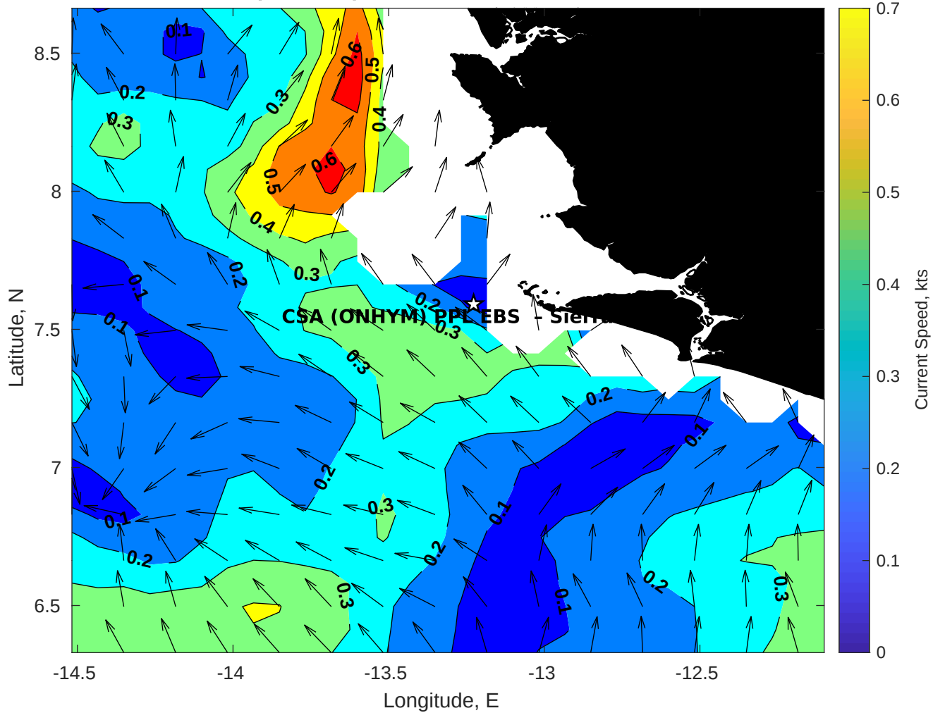
Surface Currents for CSA (ONHYM) PPL EBS - Sierra Leone at 08-Nov-2025 00:00:00
