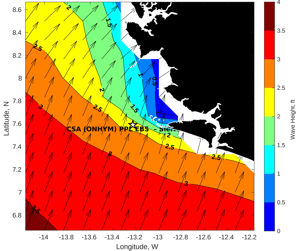
Wave Height (ft) for CSA (ONHYM) PPL EBS - Sierra Leone at 09-Nov-2025 09:00:00
