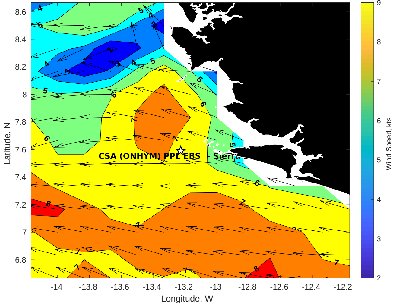
Winds (kts) for CSA (ONHYM) PPL EBS - Sierra Leone at 09-Nov-2025 09:00:00
