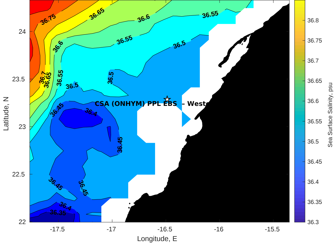
Surface Salinity for CSA (ONHYM) PPL EBS - Western Sahara at 08-Nov-2025 00:00:00
