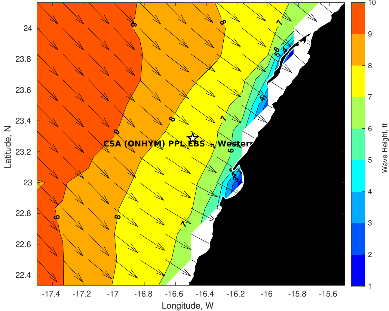
Wave Height (ft) for CSA (ONHYM) PPL EBS - Western Sahara at 09-Nov-2025 09:00:00
