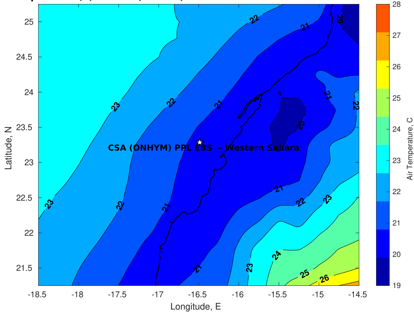
Air Temperature (C) for CSA (ONHYM) PPL EBS - Western Sahara at 09-Nov-2025
