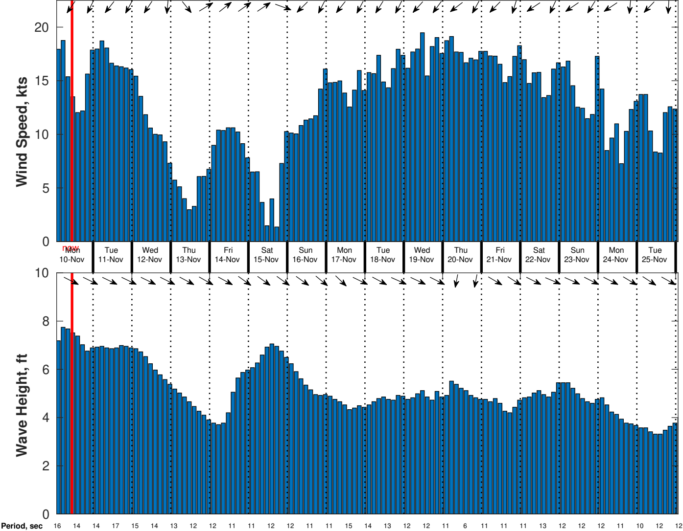
Wind & Wave Forecast for CSA (ONHYM) PPL EBS - Western Sahara from 09-Nov-2025 01:00:00 to 25-Nov-2025 01:00:00
