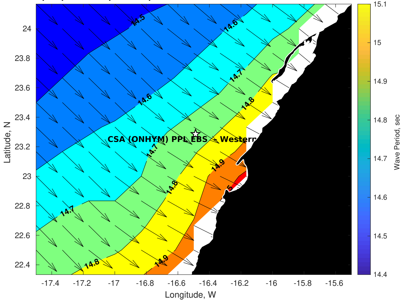
Wave Period (sec) for CSA (ONHYM) PPL EBS - Western Sahara at 09-Nov-2025 09:00:00
