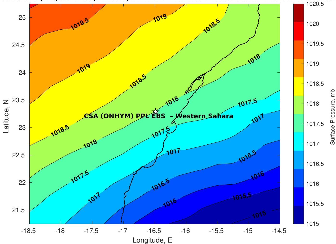
Surface Pressure (mb) for CSA (ONHYM) PPL EBS - Western Sahara at 09-Nov-2025 00:00:00
