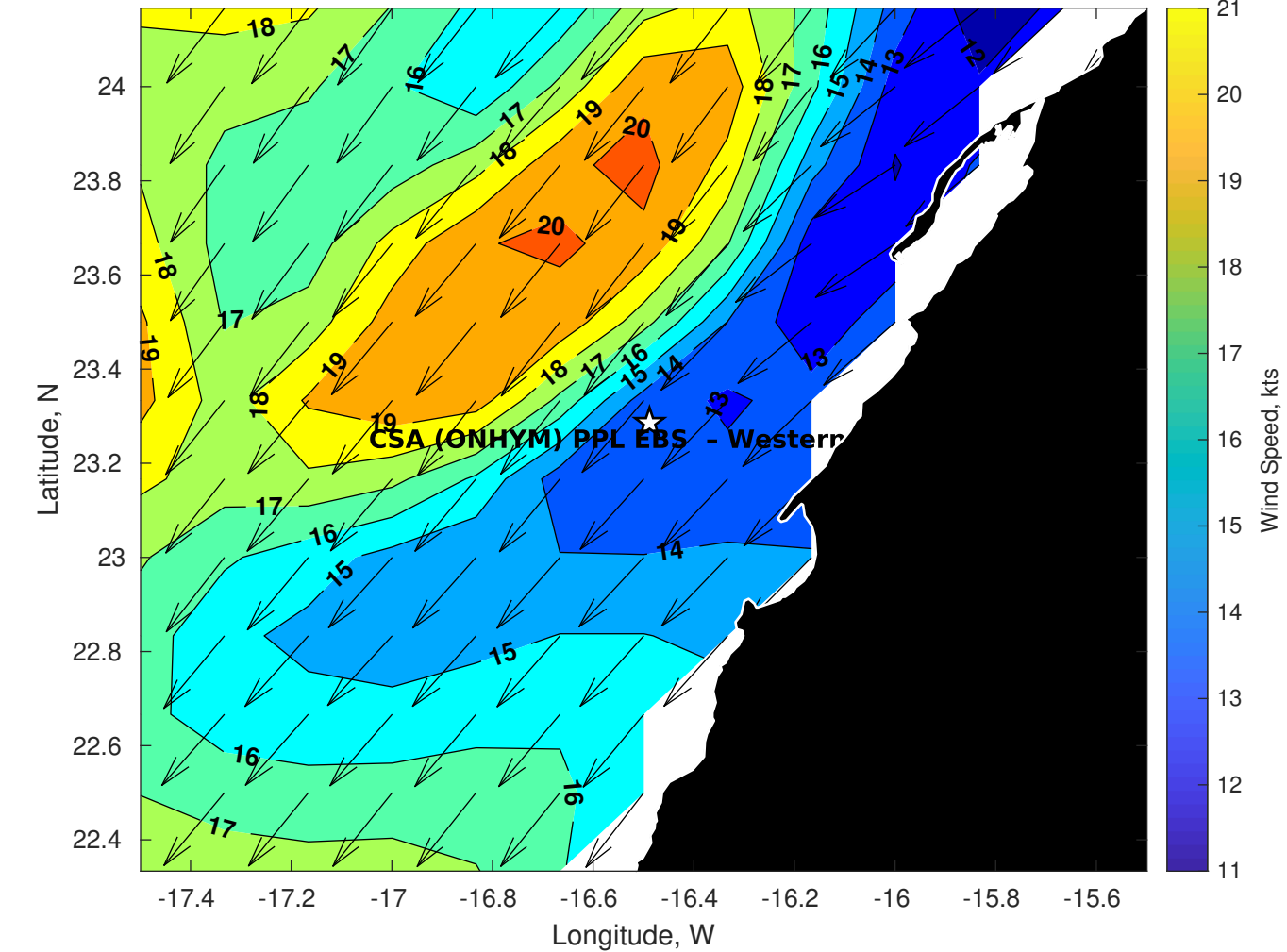
Winds (kts) for CSA (ONHYM) PPL EBS - Western Sahara at 09-Nov-2025 09:00:00
