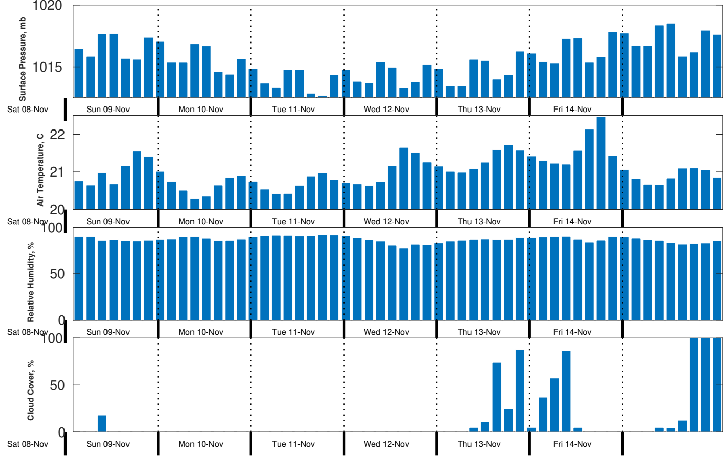
Met Forecast for CSA (ONHYM) PPL EBS - Western Sahara from 09-Nov-2025 00:00:00 to 16-Nov-2025 00:00:00
