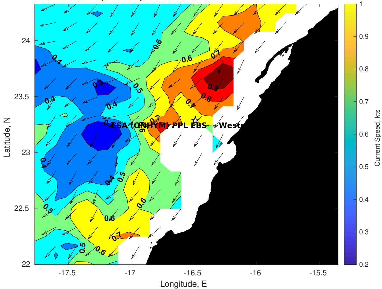
Surface Currents for CSA (ONHYM) PPL EBS - Western Sahara at 08-Nov-2025 00:00:00
