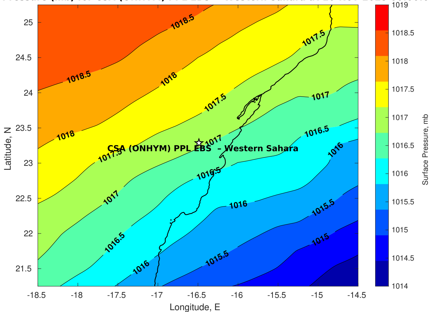
Surface Pressure (mb) for CSA (ONHYM) PPL EBS - Western Sahara at 10-Nov-2025 00:00:00
