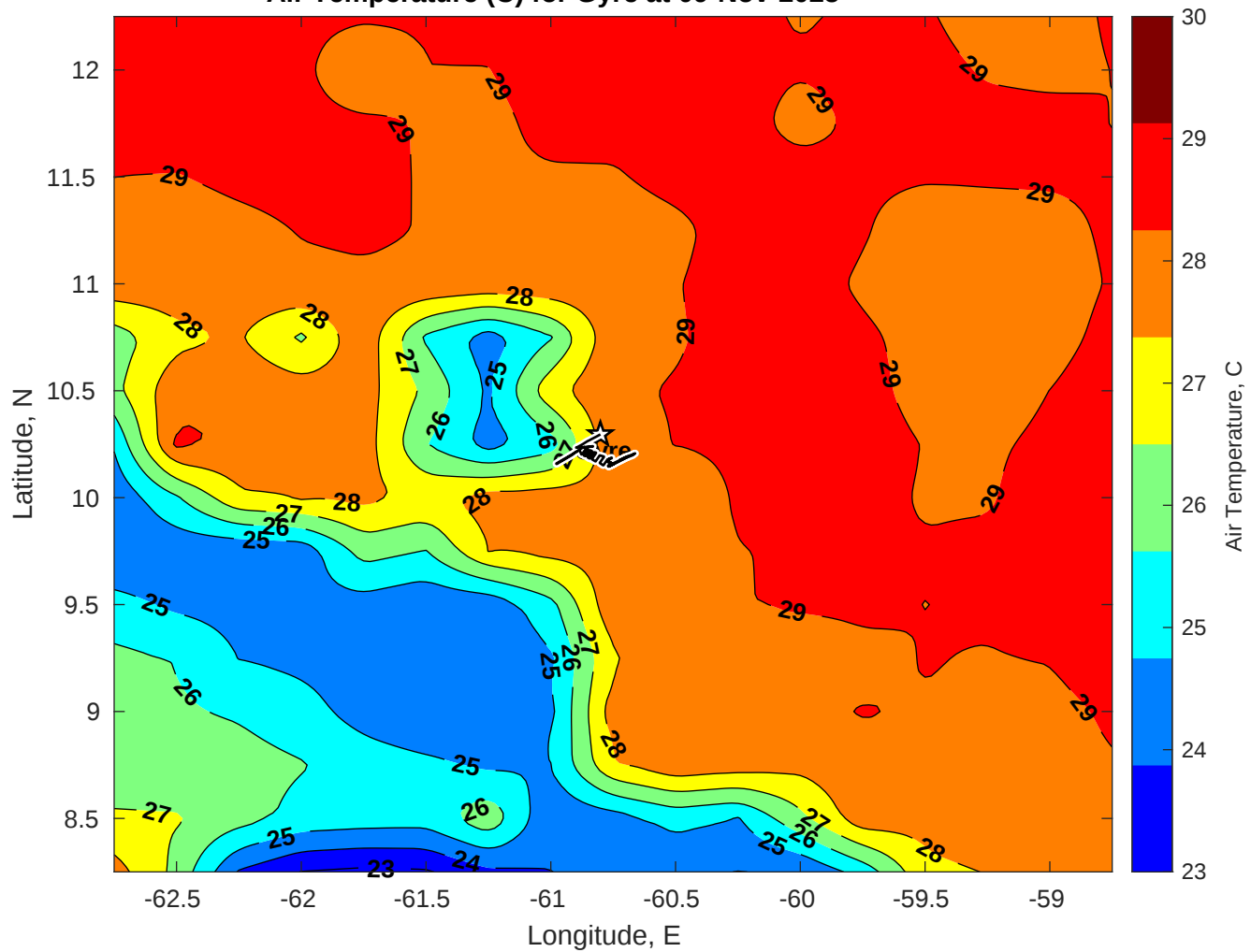
Air Temperature (C) for Gyre at 09-Nov-2025
