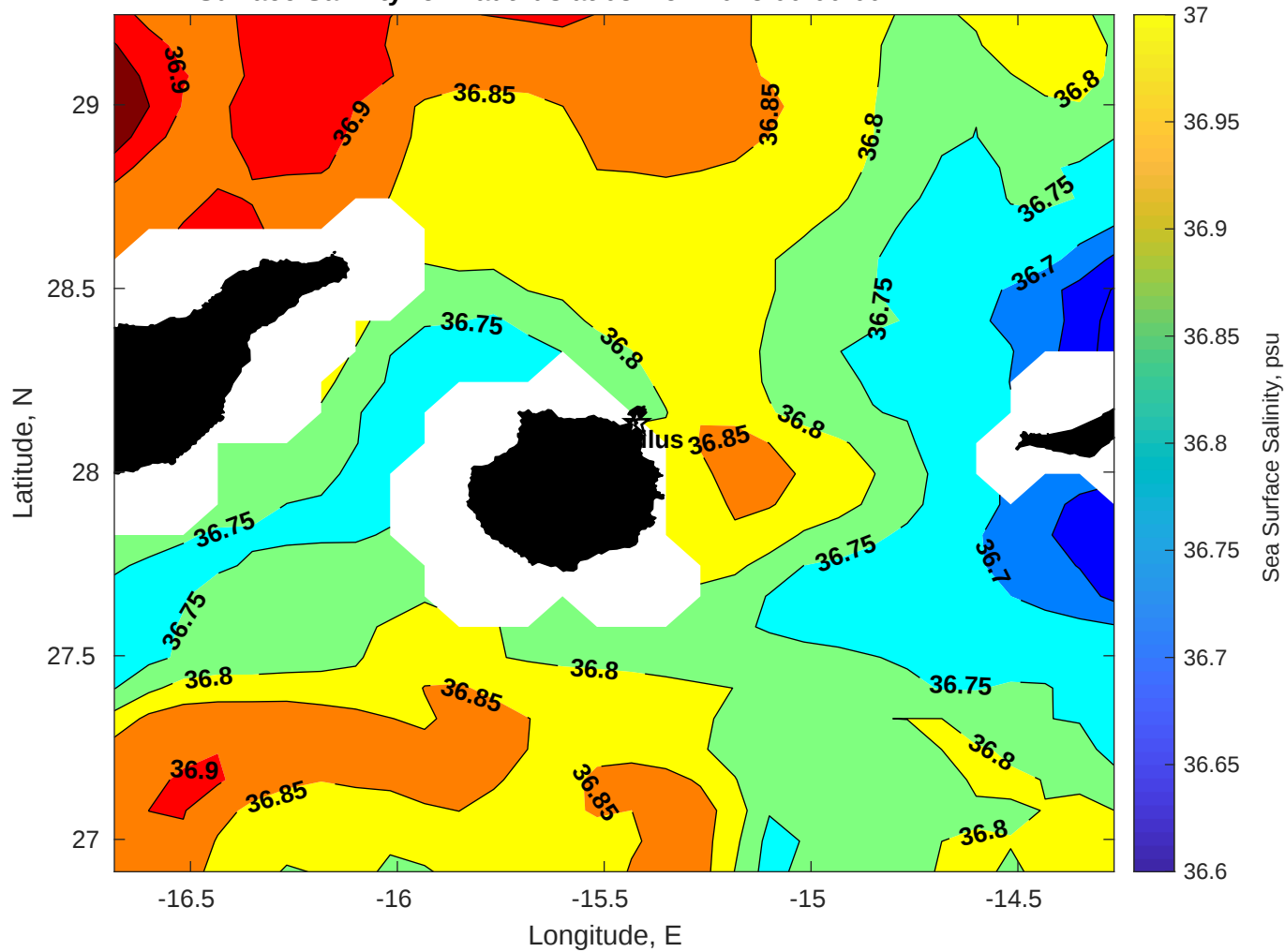
Surface Salinity for Nautilus at 08-Nov-2025 00:00:00
