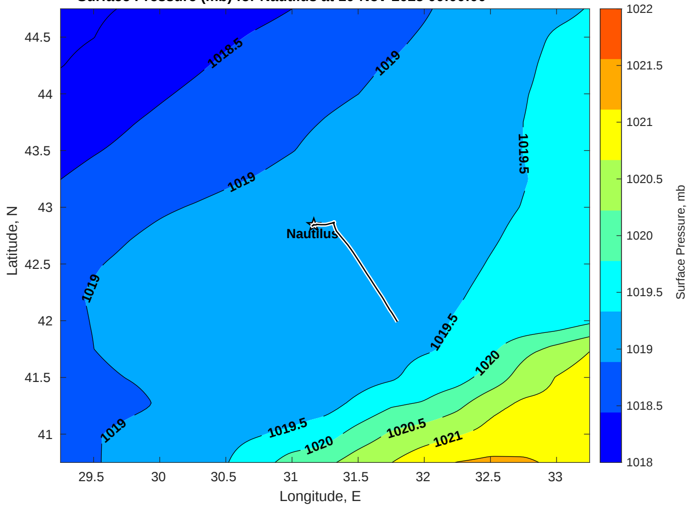
Surface Pressure (mb) for Nautilus at 10-Nov-2025 00:00:00
