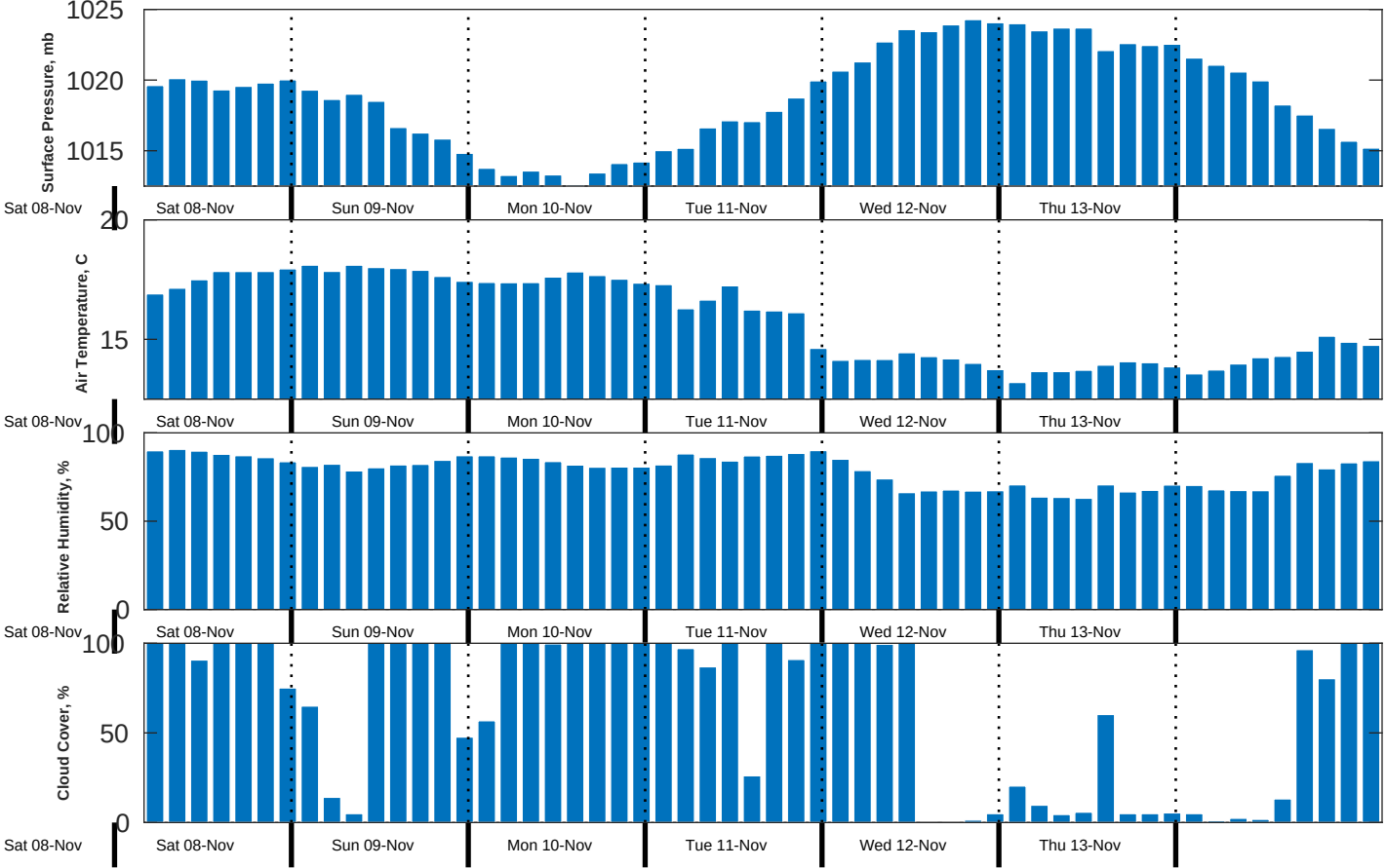
Met Forecast for Nautilus from 09-Nov-2025 00:00:00 to 16-Nov-2025 00:00:00
