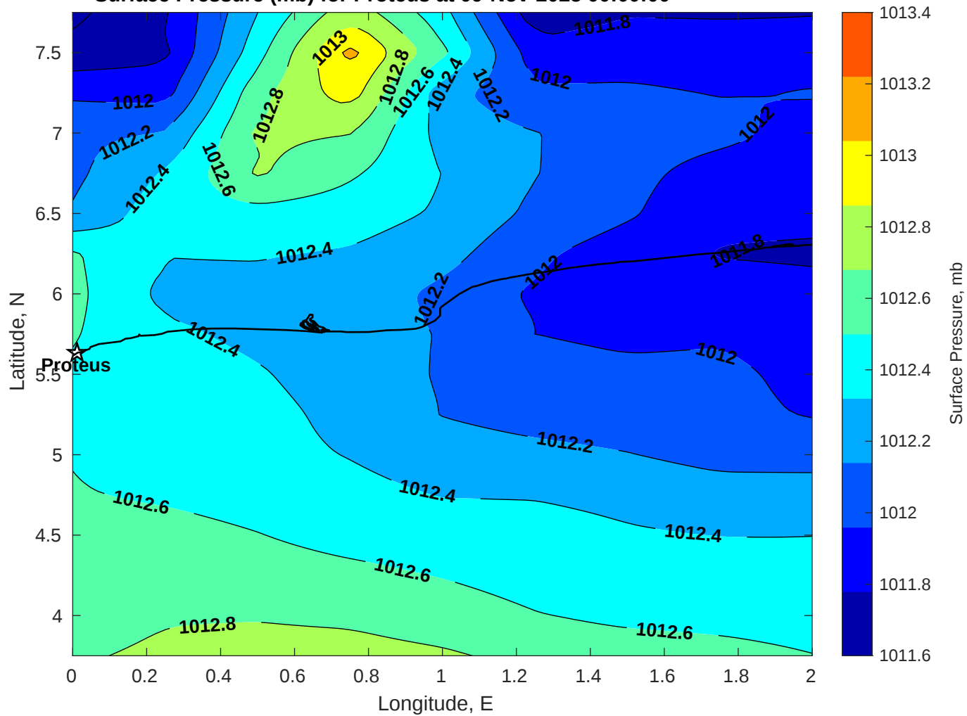
Surface Pressure (mb) for Proteus at 09-Nov-2025 00:00:00
