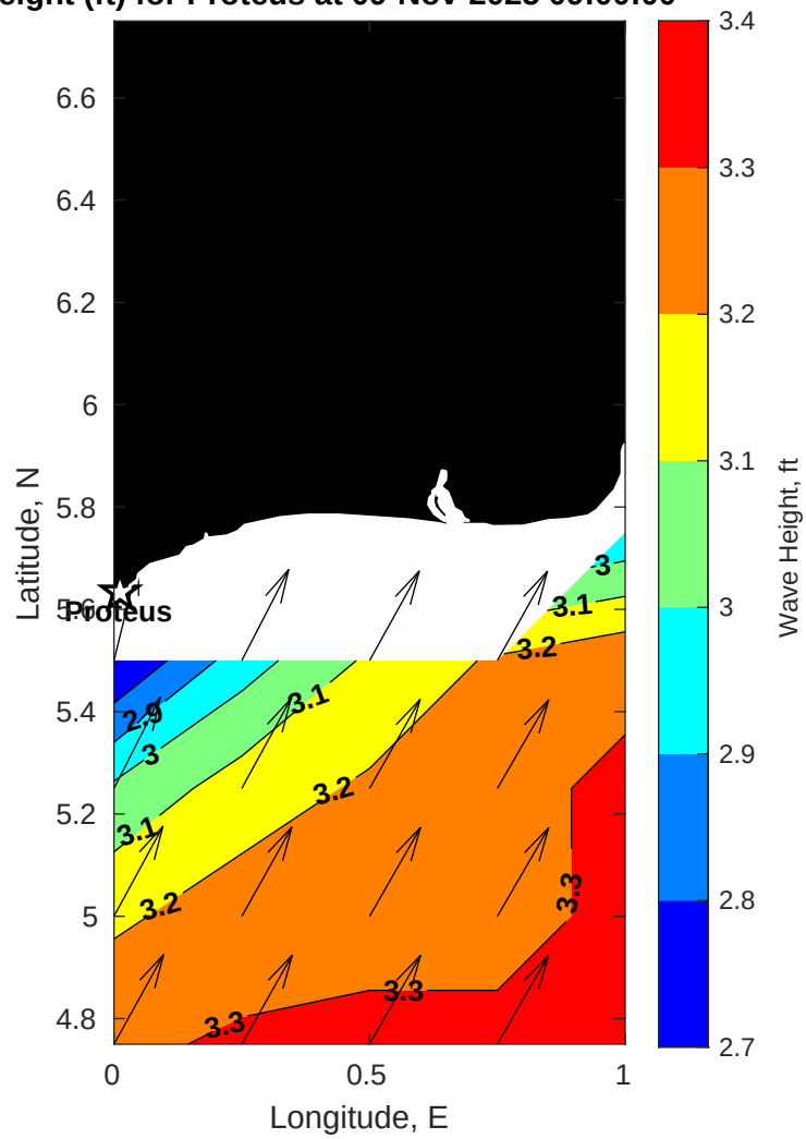
Wave Height (ft) for Proteus at 09-Nov-2025 09:00:00
