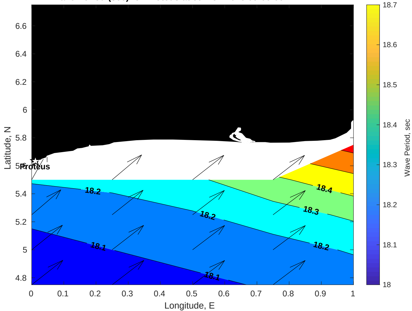
Wave Period (sec) for Proteus at 09-Nov-2025 09:00:00
