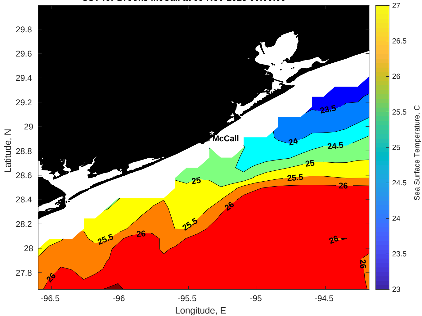
SST for Brooks McCall at 09-Nov-2025 00:00:00
