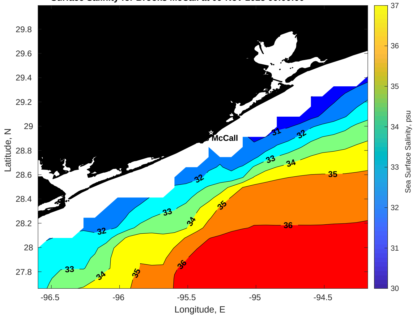
Surface Salinity for Brooks McCall at 09-Nov-2025 00:00:00
