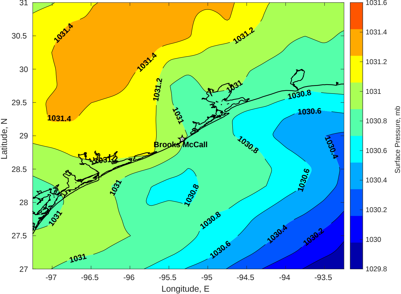
Surface Pressure (mb) for Brooks McCall at 11-Nov-2025 00:00:00
