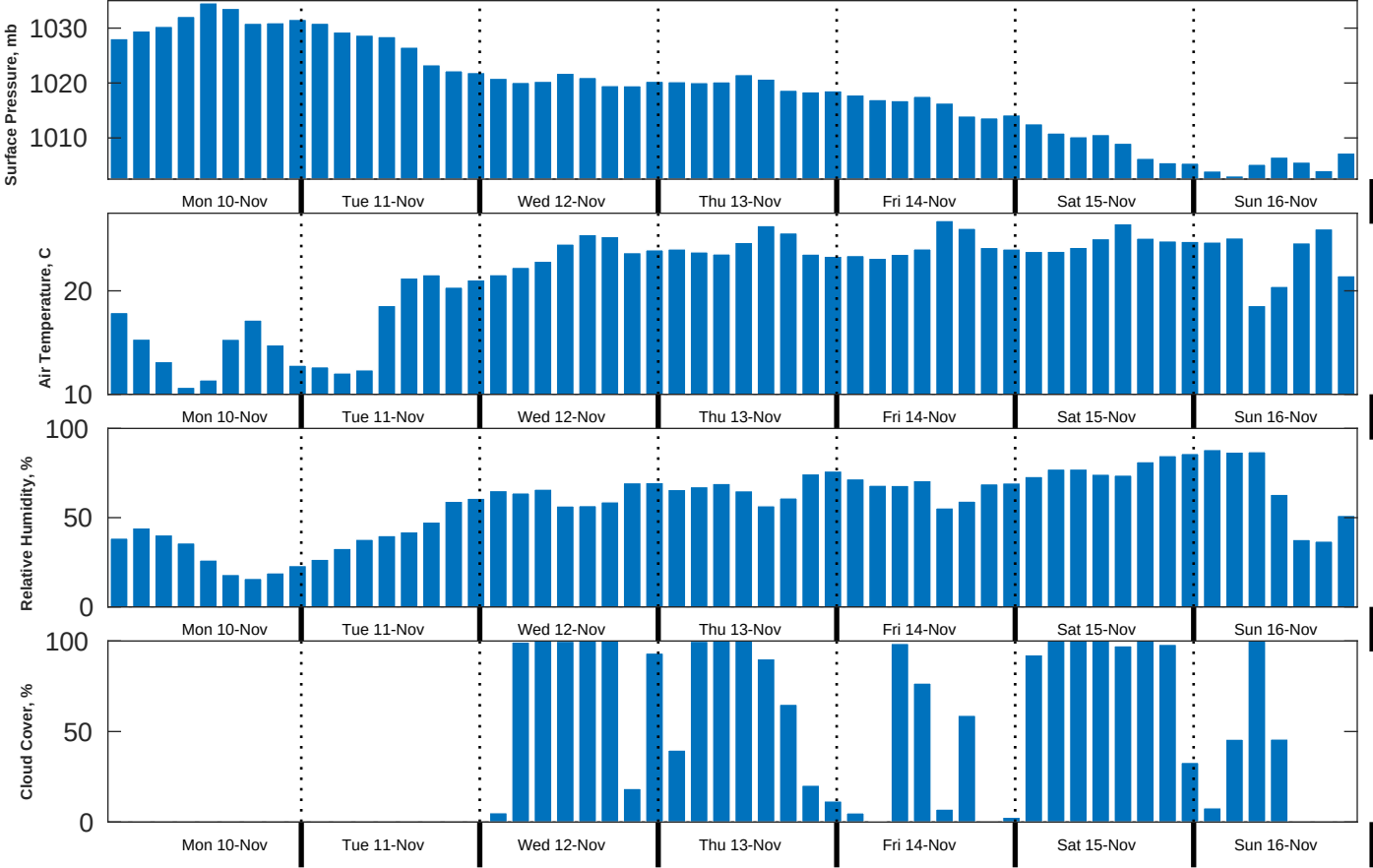
Met Forecast for Brooks McCall from 10-Nov-2025 00:00:00 to 17-Nov-2025 00:00:00
