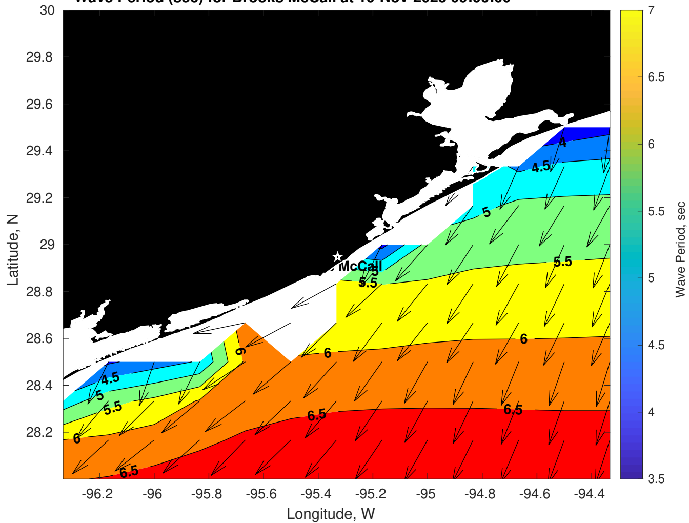
Wave Period (sec) for Brooks McCall at 10-Nov-2025 09:00:00
