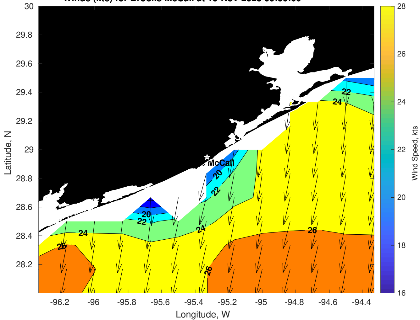
Winds (kts) for Brooks McCall at 10-Nov-2025 09:00:00
