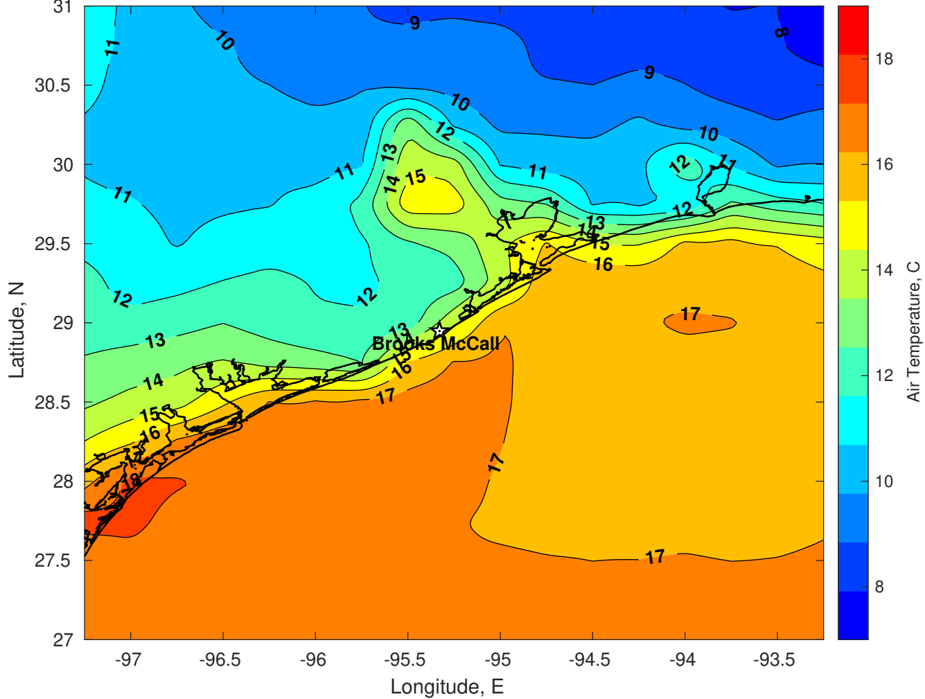
Air Temperature (C) for Brooks McCall at 10-Nov-2025
