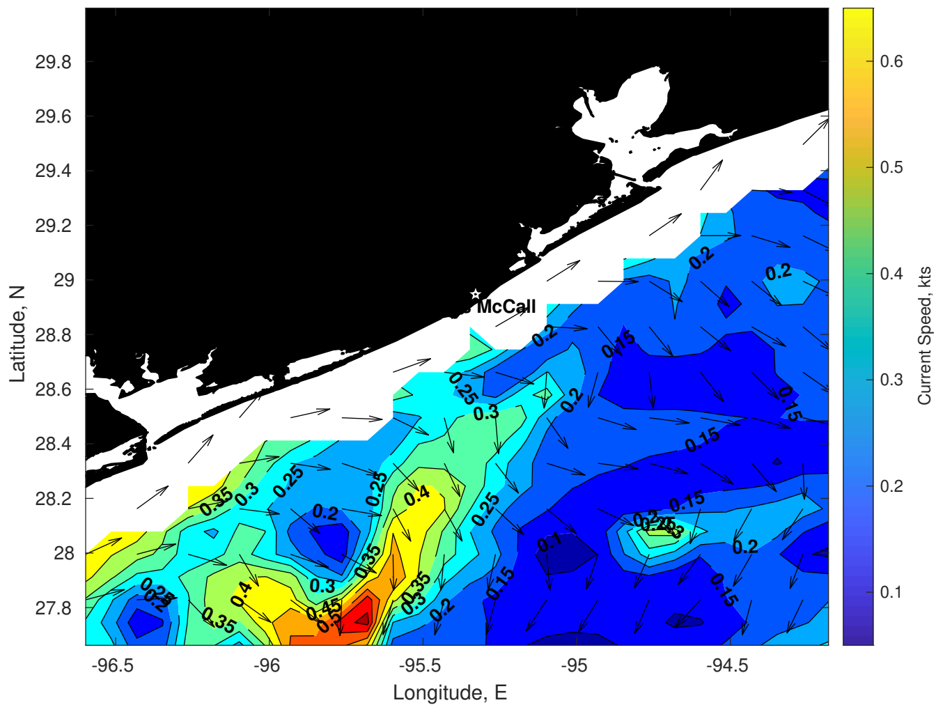
Surface Currents for Brooks McCall at 09-Nov-2025 00:00:00
