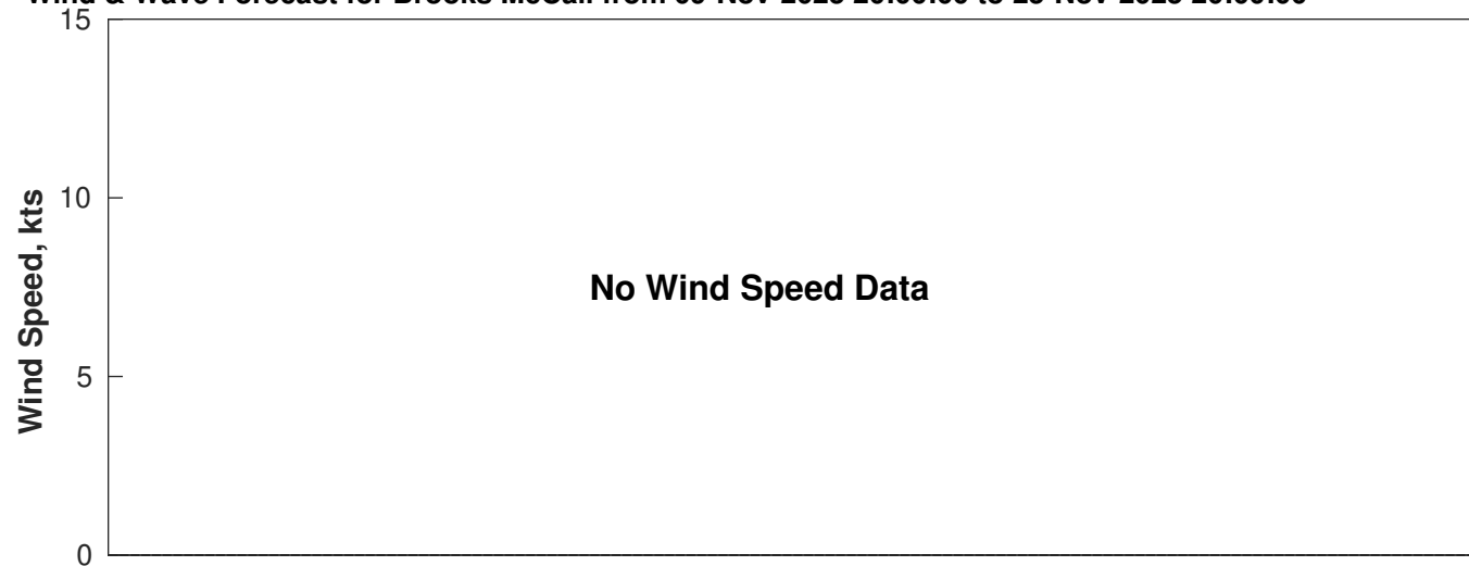
Wind & Wave Forecast for Brooks McCall from 09-Nov-2025 20:00:00 to 25-Nov-2025 20:00:00
