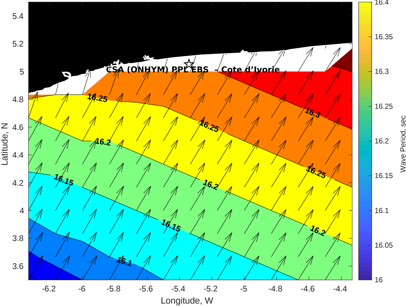
Wave Period (sec) for CSA (ONHYM) PPL EBS - Cote d'Ivoire at 10-Nov-2025 09:00:00
