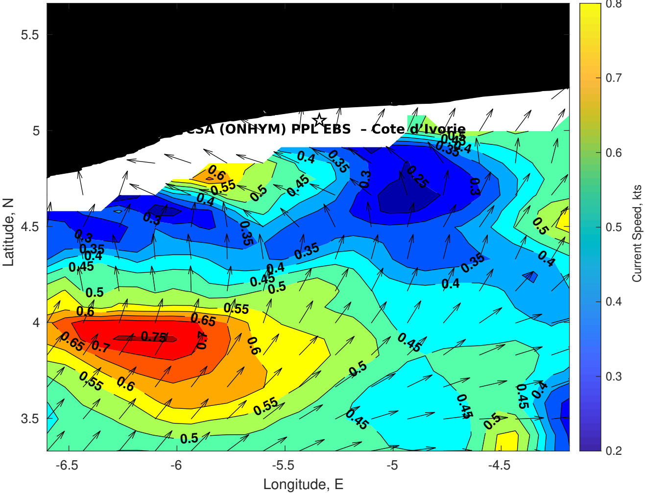
Surface Currents for CSA (ONHYM) PPL EBS - Cote d'Ivoire at 09-Nov-2025 00:00:00
