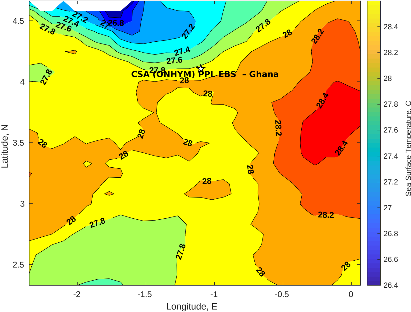
SST for CSA (ONHYM) PPL EBS - Ghana at 09-Nov-2025 00:00:00
