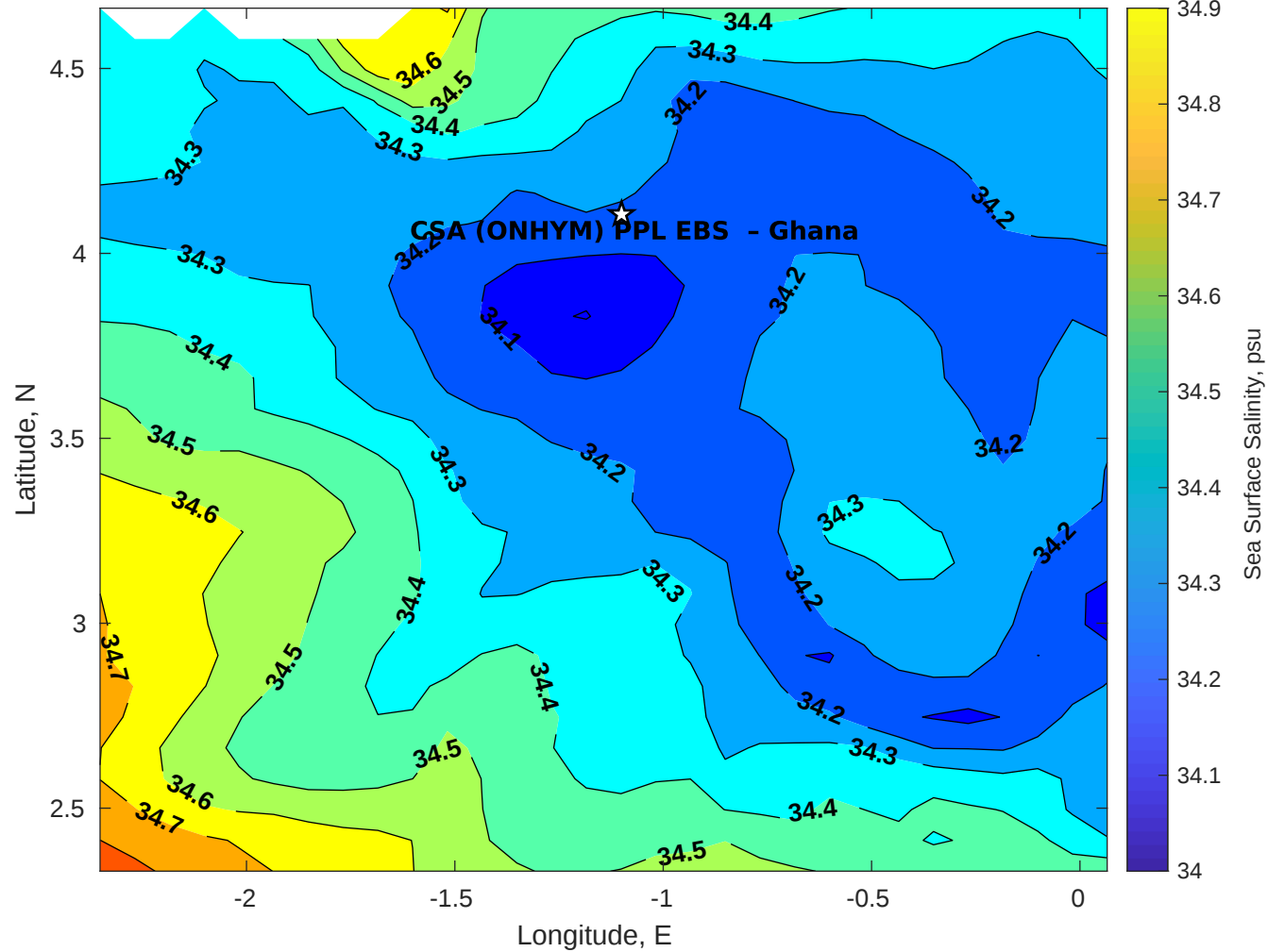
Surface Salinity for CSA (ONHYM) PPL EBS - Ghana at 09-Nov-2025 00:00:00
