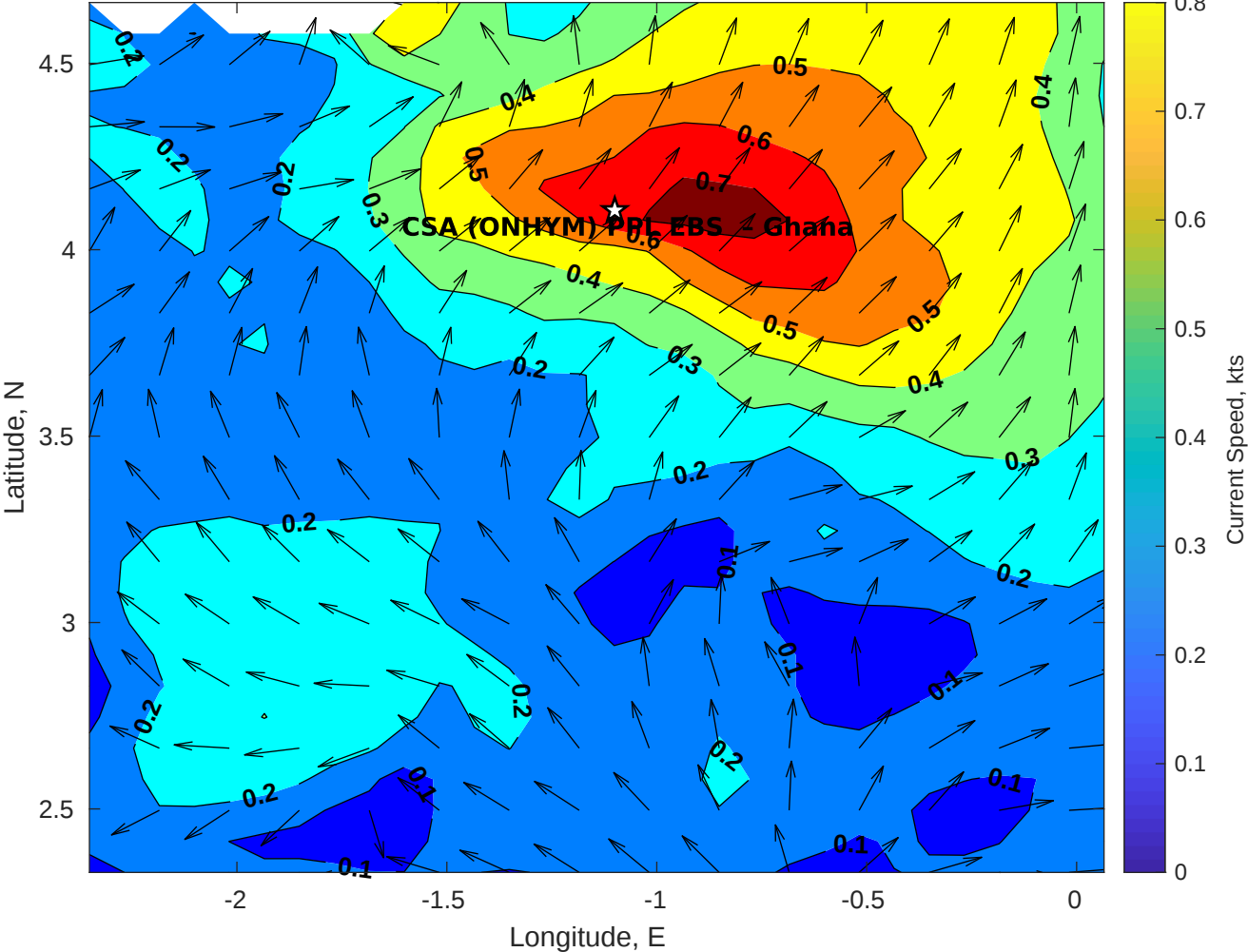
Surface Currents for CSA (ONHYM) PPL EBS - Ghana at 09-Nov-2025 00:00:00
