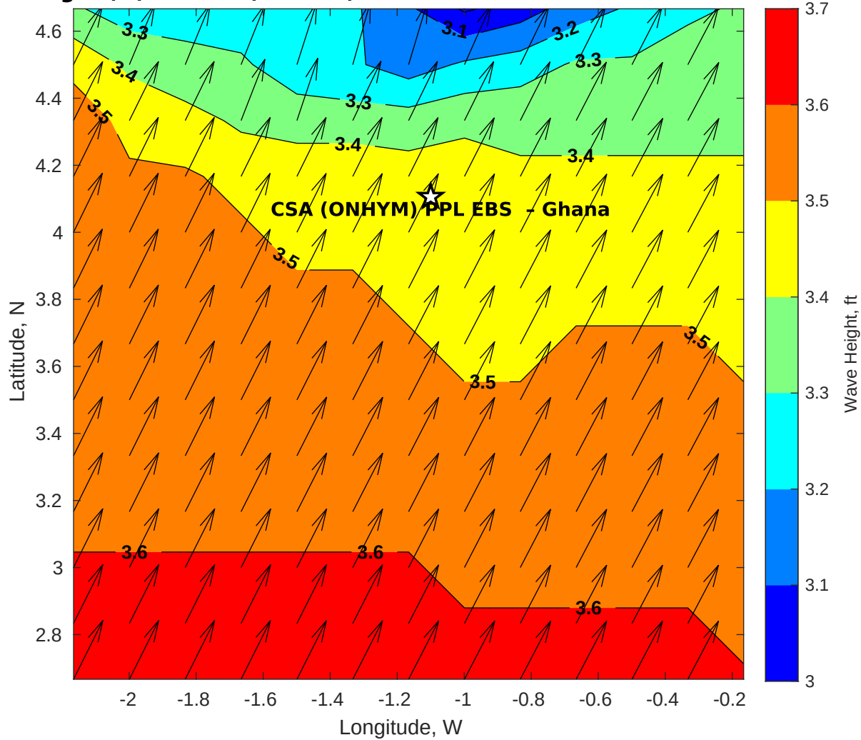
Wave Height (ft) for CSA (ONHYM) PPL EBS - Ghana at 10-Nov-2025 09:00:00
