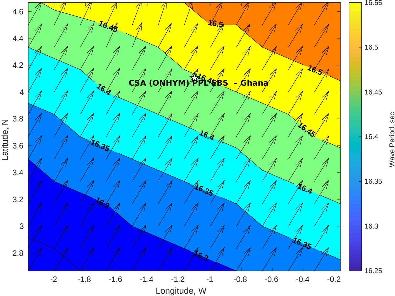
Wave Period (sec) for CSA (ONHYM) PPL EBS - Ghana at 10-Nov-2025 09:00:00
