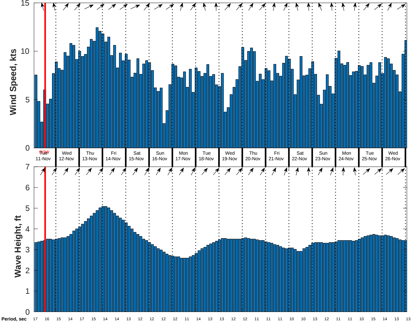
Wind & Wave Forecast for CSA (ONHYM) PPL EBS - Ghana from 10-Nov-2025 02:00:00 to 26-Nov-2025 02:00:00
