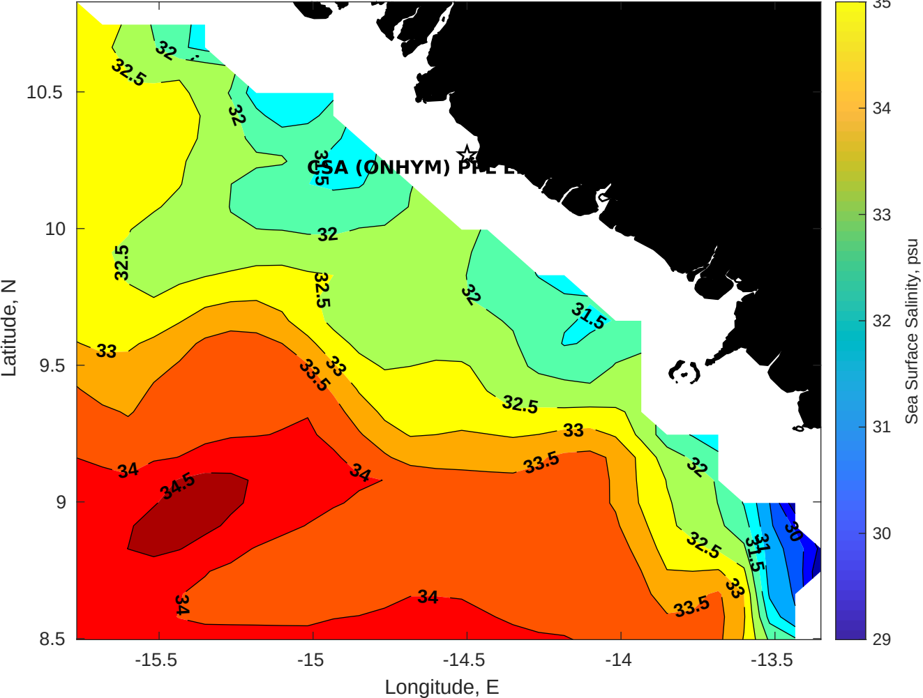
Surface Salinity for CSA (ONHYM) PPL EBS - Guinea at 09-Nov-2025 00:00:00
