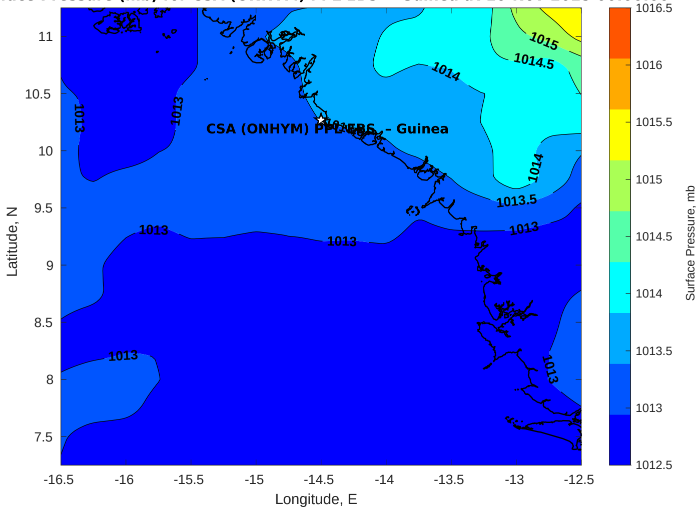
Surface Pressure (mb) for CSA (ONHYM) PPL EBS - Guinea at 10-Nov-2025 00:00:00
