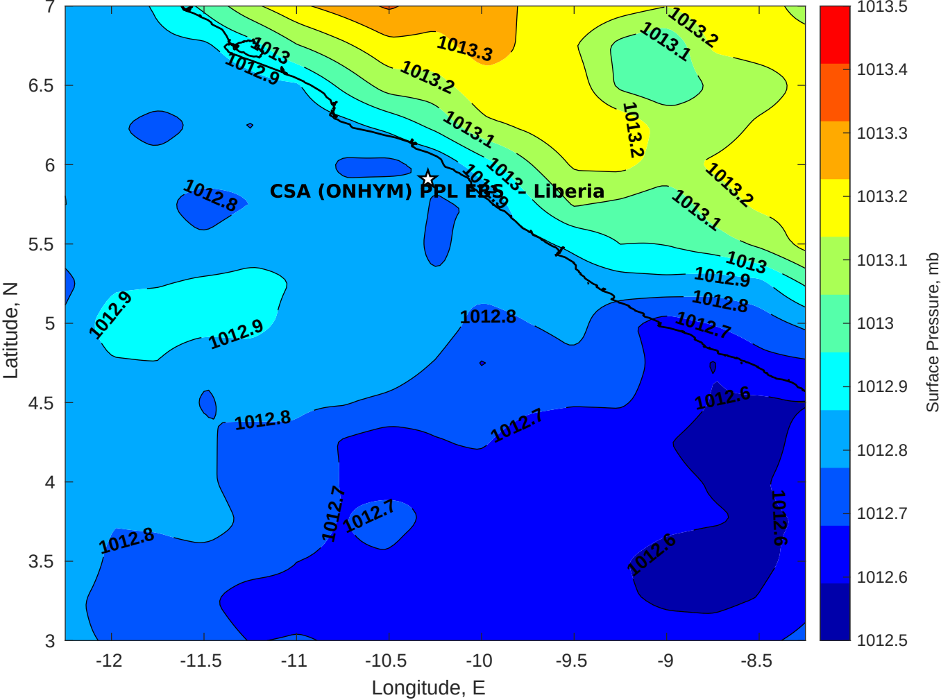
Surface Pressure (mb) for CSA (ONHYM) PPL EBS - Liberia at 12-Nov-2025 00:00:00
