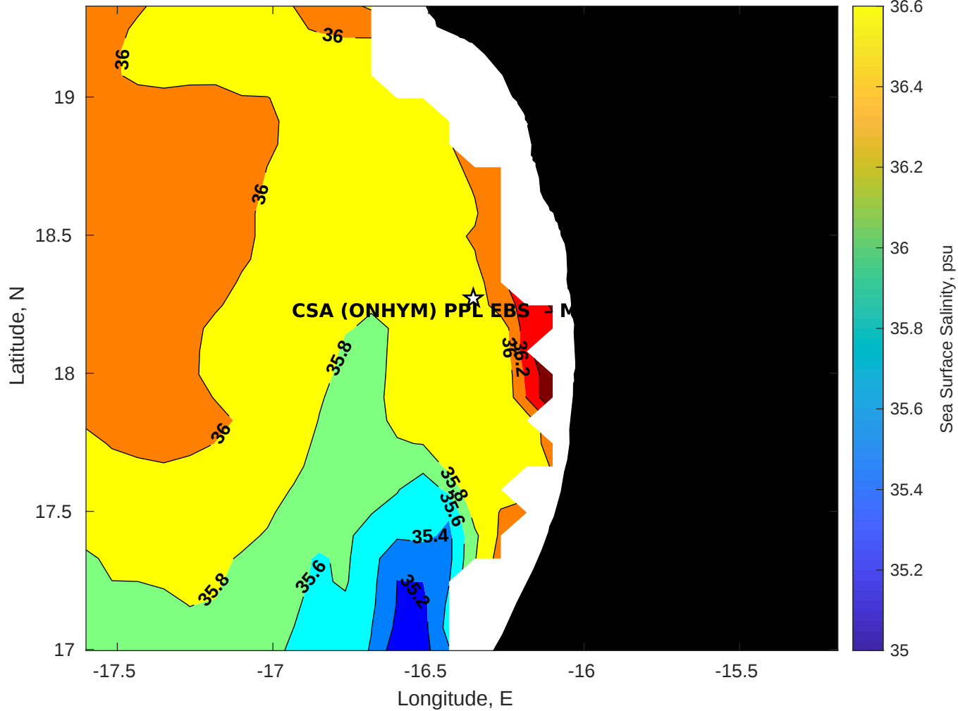
Surface Salinity for CSA (ONHYM) PPL EBS - Mauritania at 09-Nov-2025 00:00:00
