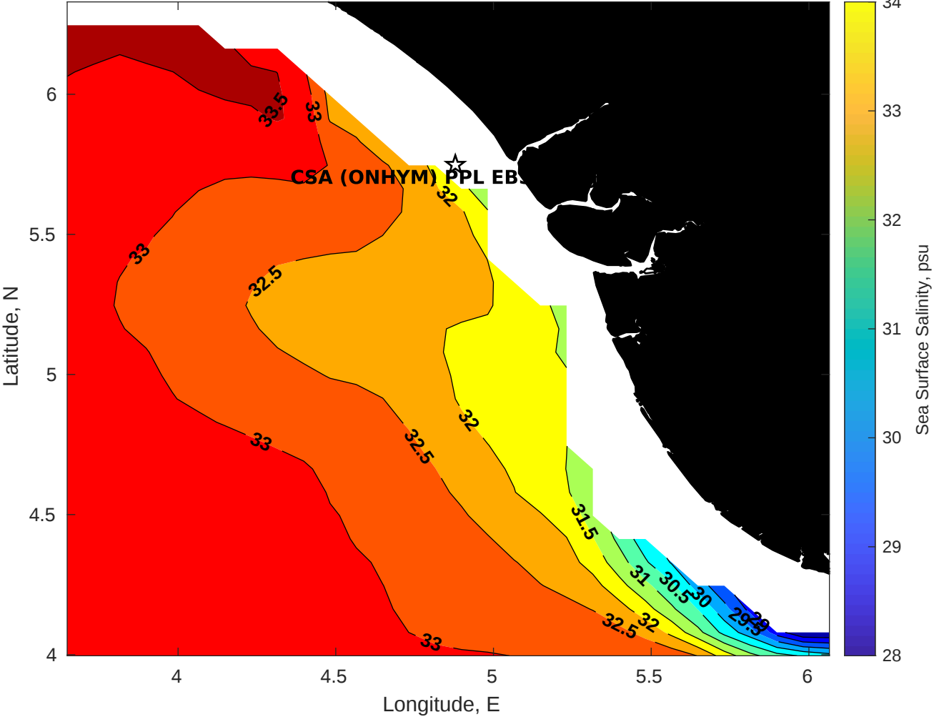
Surface Salinity for CSA (ONHYM) PPL EBS - Nigeria at 09-Nov-2025 00:00:00
