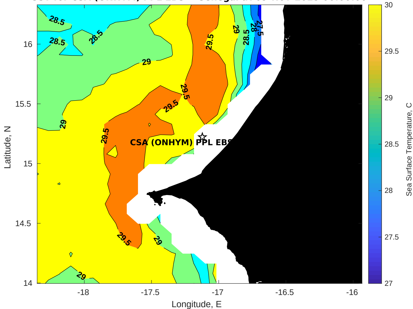
SST for CSA (ONHYM) PPL EBS - Senegal at 09-Nov-2025 00:00:00
