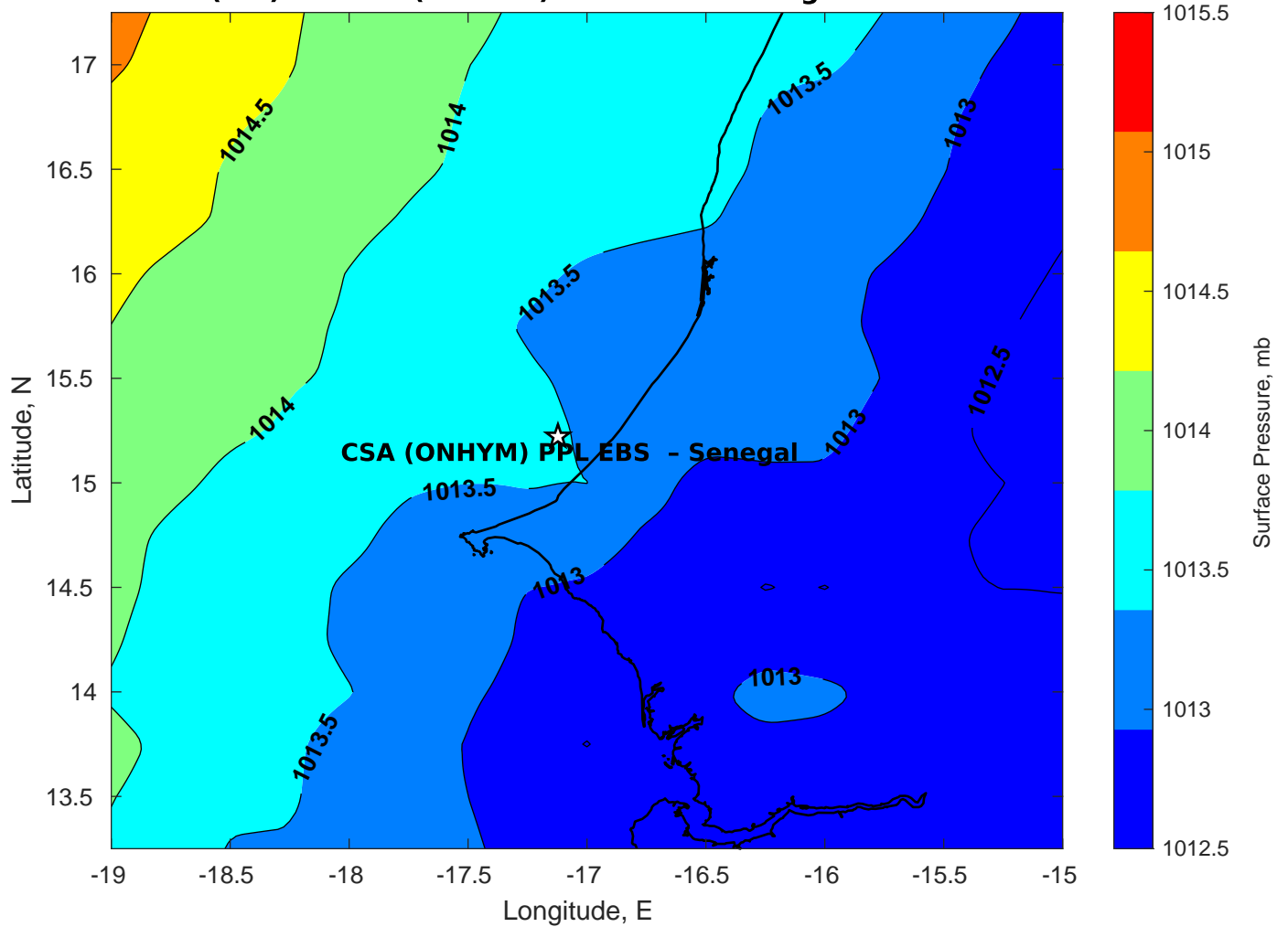
Surface Pressure (mb) for CSA (ONHYM) PPL EBS - Senegal at 10-Nov-2025 00:00:00
