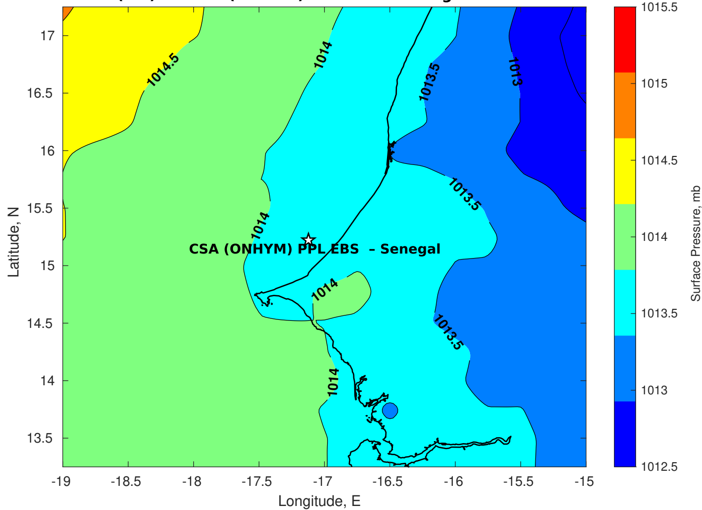
Surface Pressure (mb) for CSA (ONHYM) PPL EBS - Senegal at 11-Nov-2025 00:00:00
