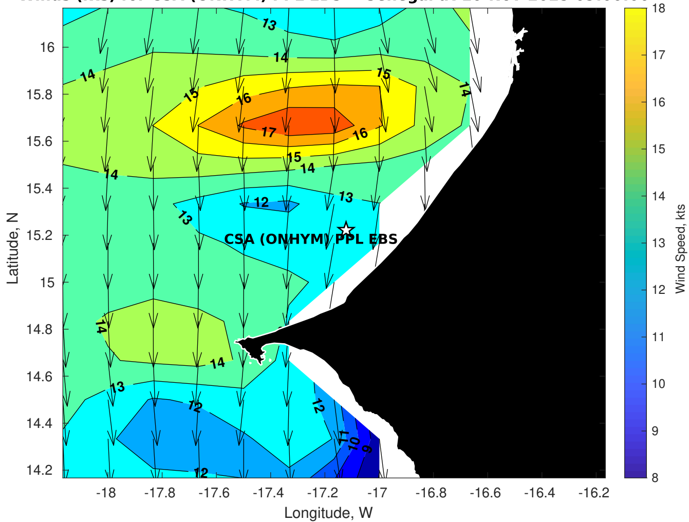
Winds (kts) for CSA (ONHYM) PPL EBS - Senegal at 10-Nov-2025 09:00:00
