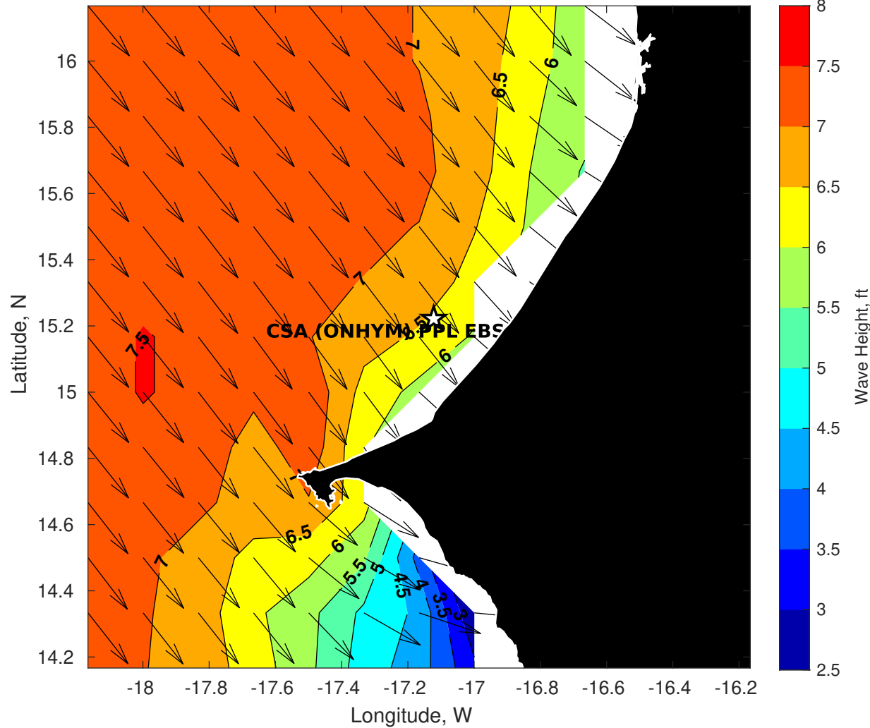
Wave Height (ft) for CSA (ONHYM) PPL EBS - Senegal at 10-Nov-2025 09:00:00
