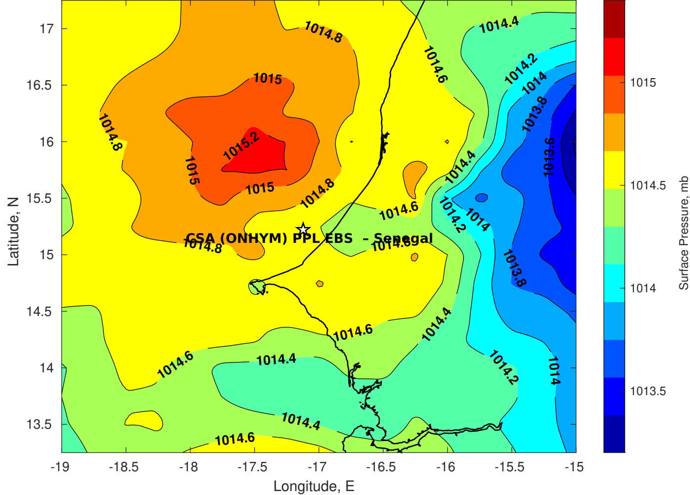
Surface Pressure (mb) for CSA (ONHYM) PPL EBS - Senegal at 12-Nov-2025 00:00:00
