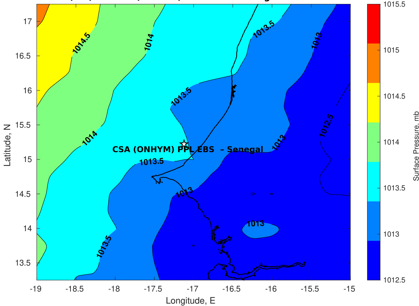
Surface Pressure (mb) for CSA (ONHYM) PPL EBS - Senegal at 10-Nov-2025 00:00:00
