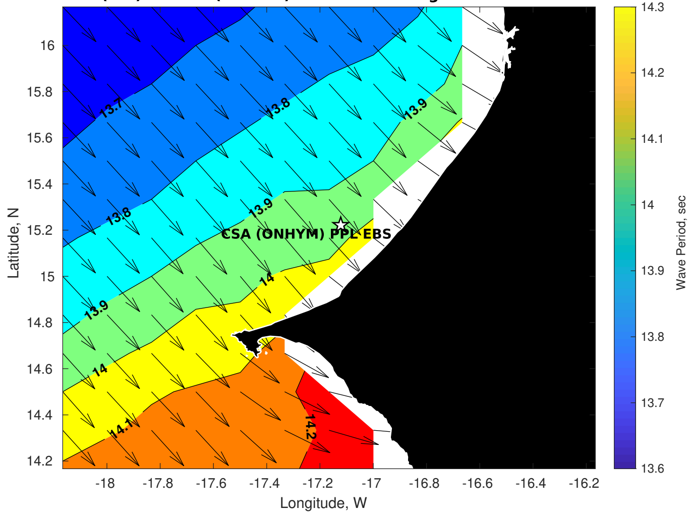
Wave Period (sec) for CSA (ONHYM) PPL EBS - Senegal at 10-Nov-2025 09:00:00
