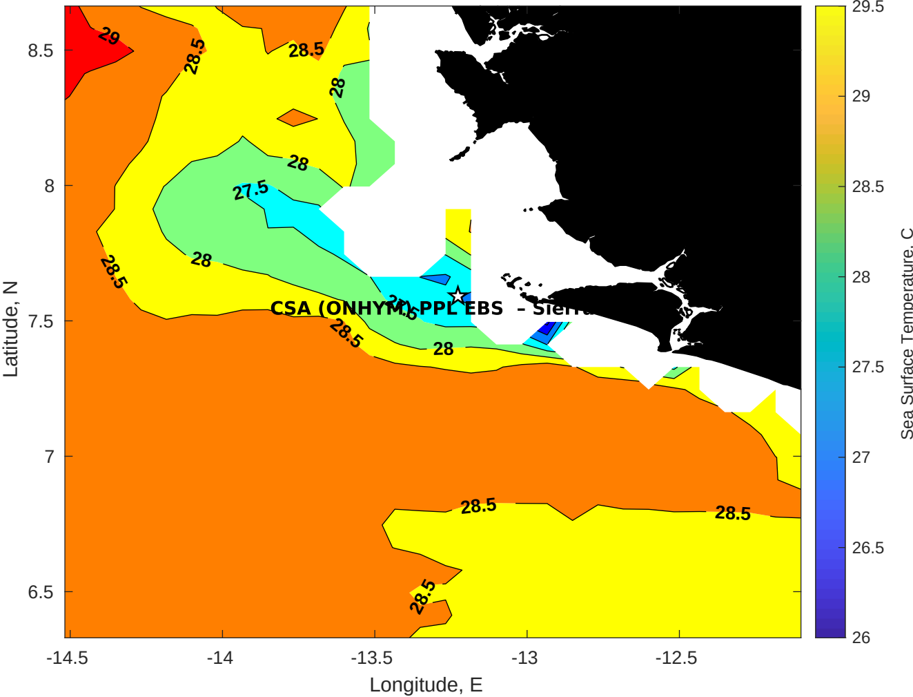
SST for CSA (ONHYM) PPL EBS - Sierra Leone at 09-Nov-2025 00:00:00
