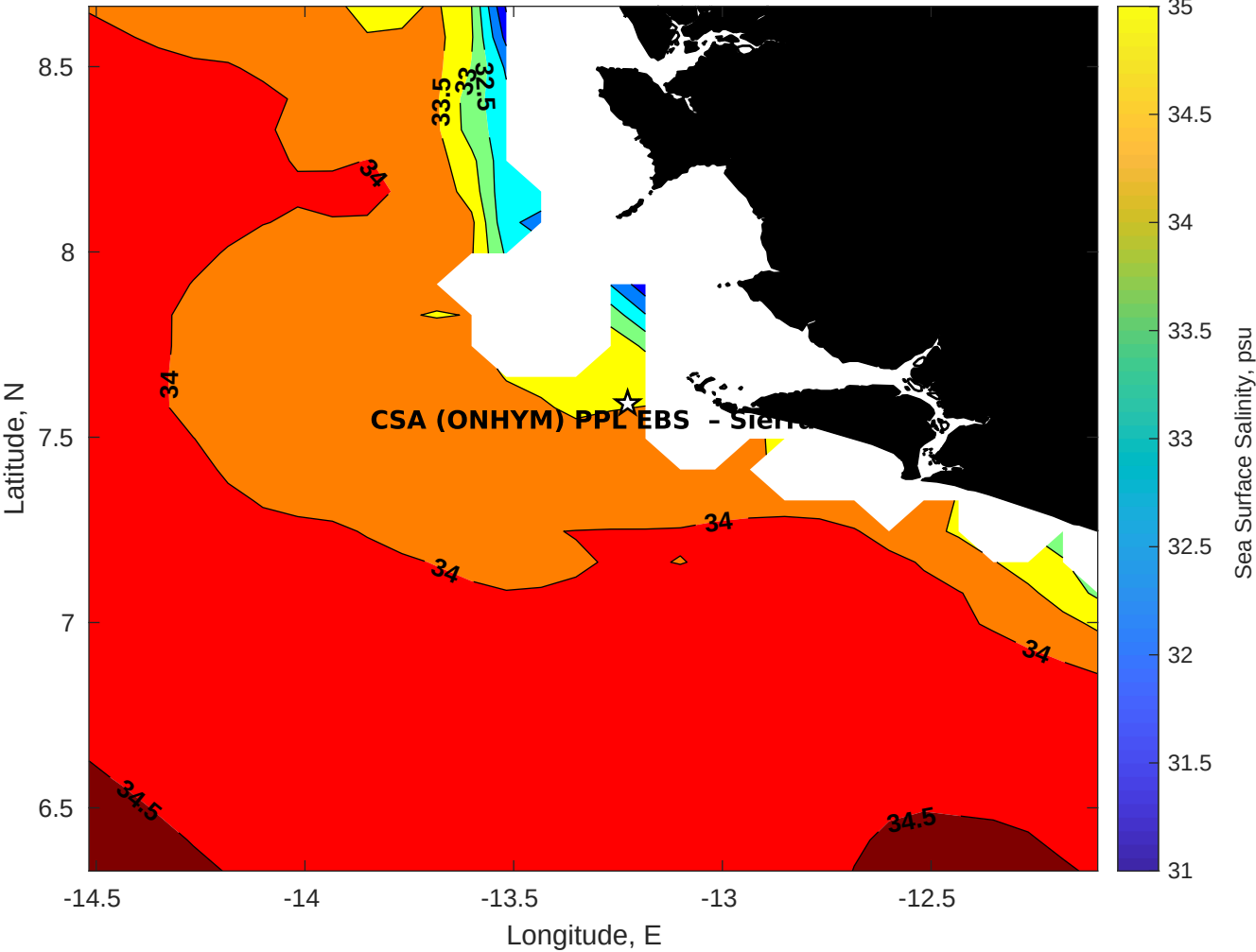
Surface Salinity for CSA (ONHYM) PPL EBS - Sierra Leone at 09-Nov-2025 00:00:00
