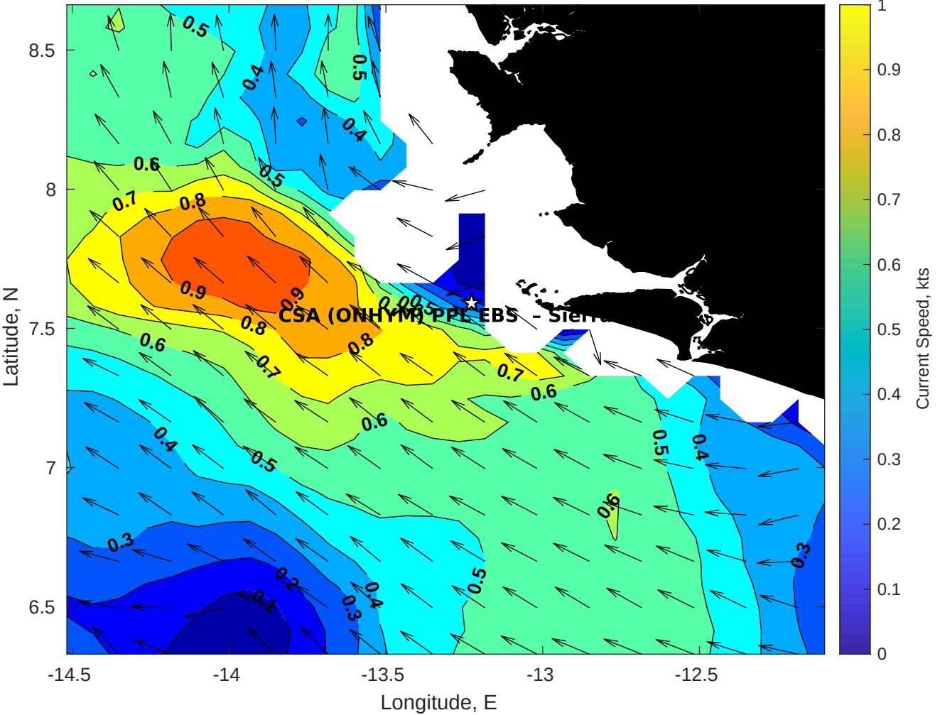
Surface Currents for CSA (ONHYM) PPL EBS - Sierra Leone at 09-Nov-2025 00:00:00
