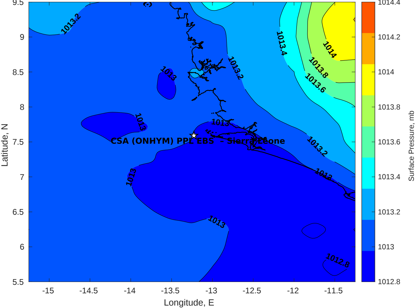
Surface Pressure (mb) for CSA (ONHYM) PPL EBS - Sierra Leone at 12-Nov-2025 00:00:00
