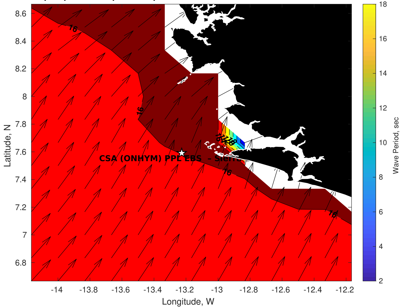
Wave Period (sec) for CSA (ONHYM) PPL EBS - Sierra Leone at 10-Nov-2025 09:00:00
