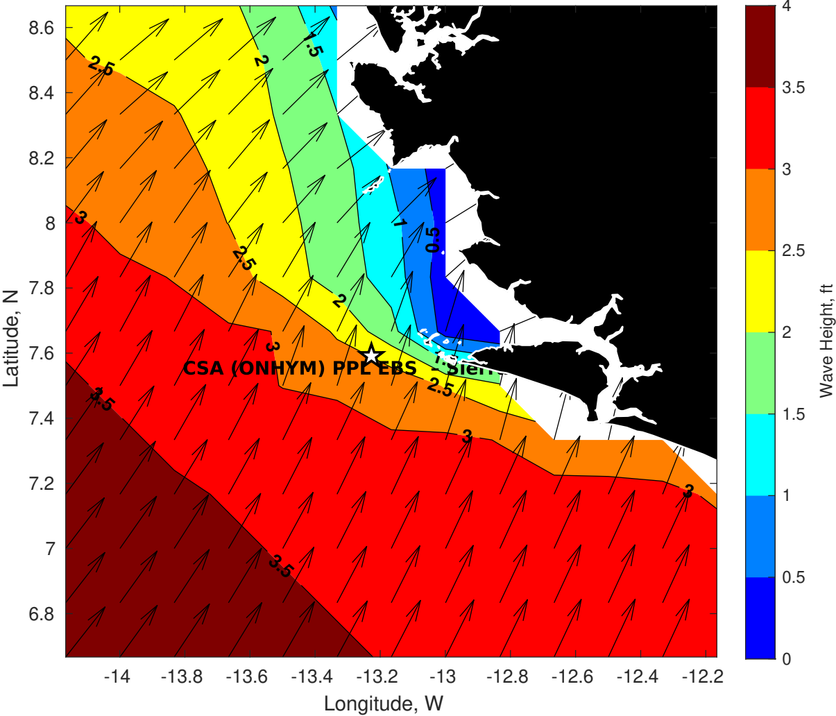
Wave Height (ft) for CSA (ONHYM) PPL EBS - Sierra Leone at 10-Nov-2025 09:00:00
