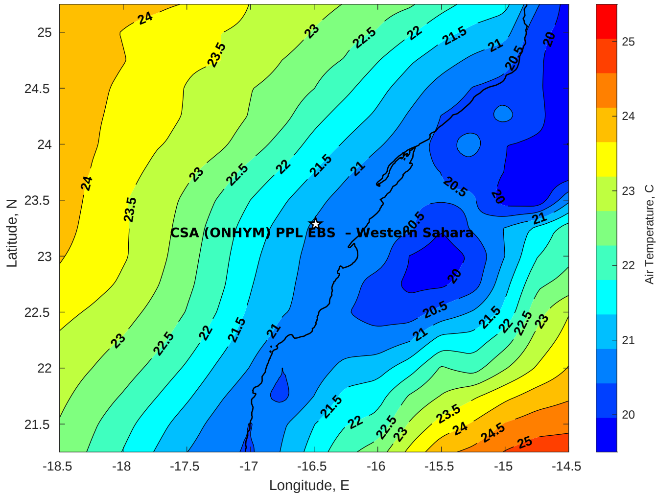
Air Temperature (C) for CSA (ONHYM) PPL EBS - Western Sahara at 10-Nov-2025
