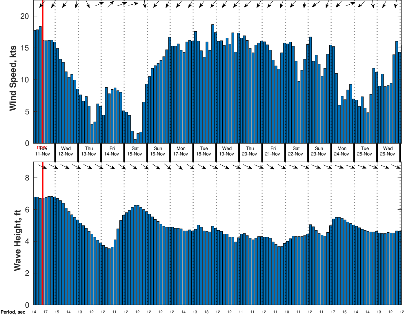
Wind & Wave Forecast for CSA (ONHYM) PPL EBS - Western Sahara from 10-Nov-2025 01:00:00 to 26-Nov-2025 01:00:00
