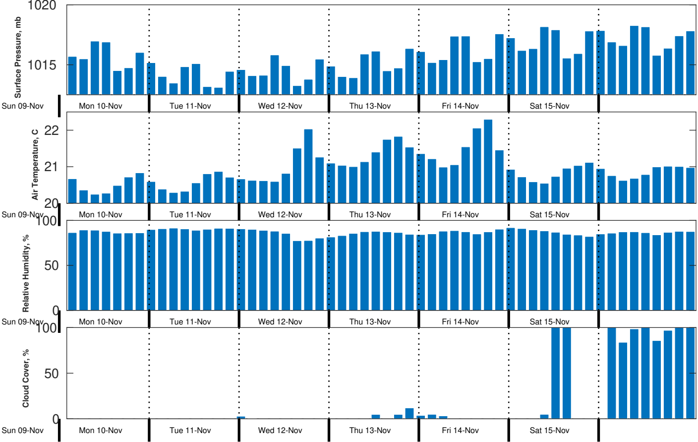
Met Forecast for CSA (ONHYM) PPL EBS - Western Sahara from 10-Nov-2025 00:00:00 to 17-Nov-2025 00:00:00
