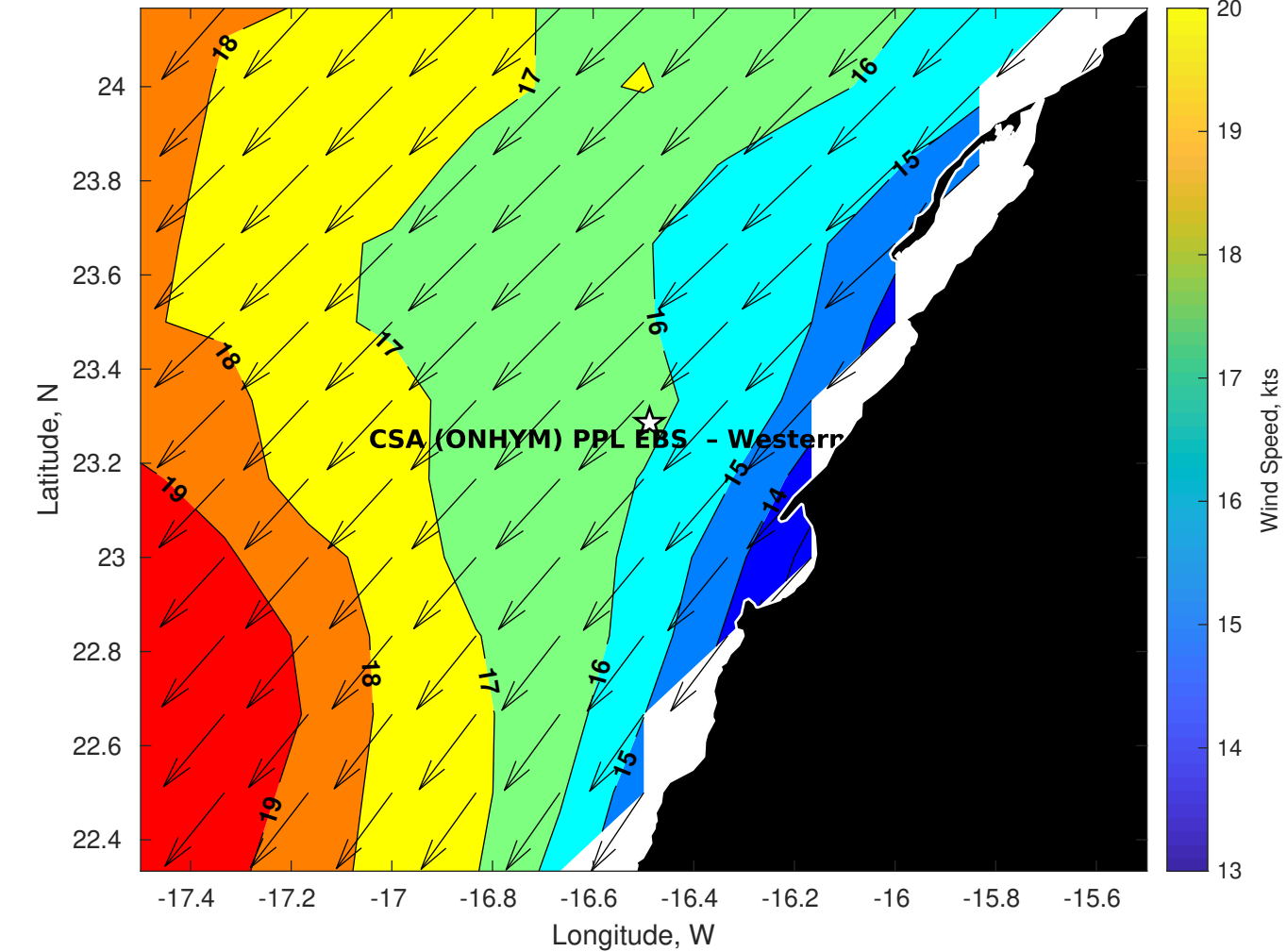
Winds (kts) for CSA (ONHYM) PPL EBS - Western Sahara at 10-Nov-2025 09:00:00
