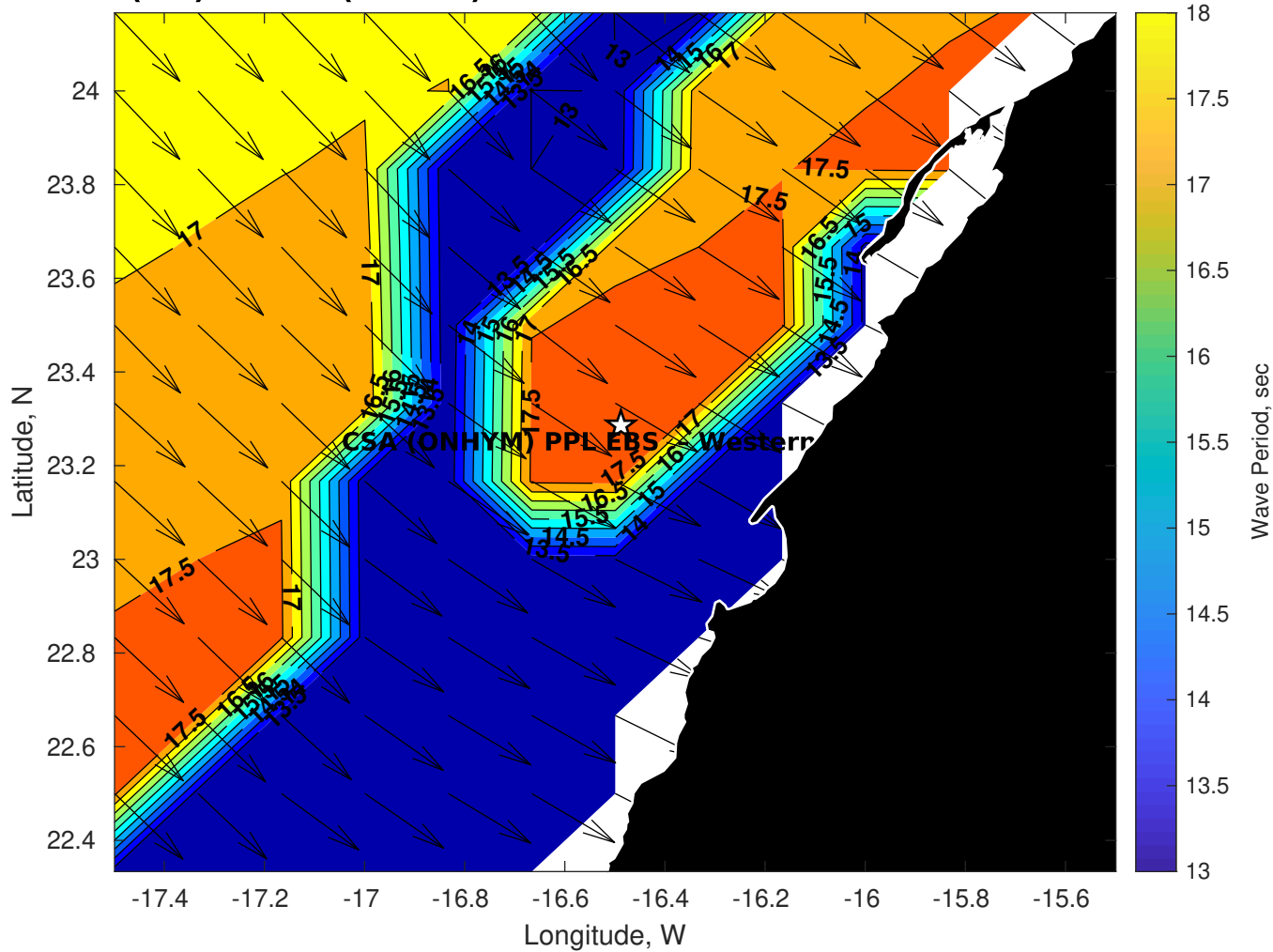
Wave Period (sec) for CSA (ONHYM) PPL EBS - Western Sahara at 10-Nov-2025 09:00:00
