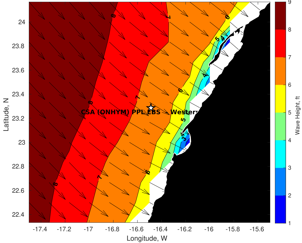
Wave Height (ft) for CSA (ONHYM) PPL EBS - Western Sahara at 10-Nov-2025 09:00:00
