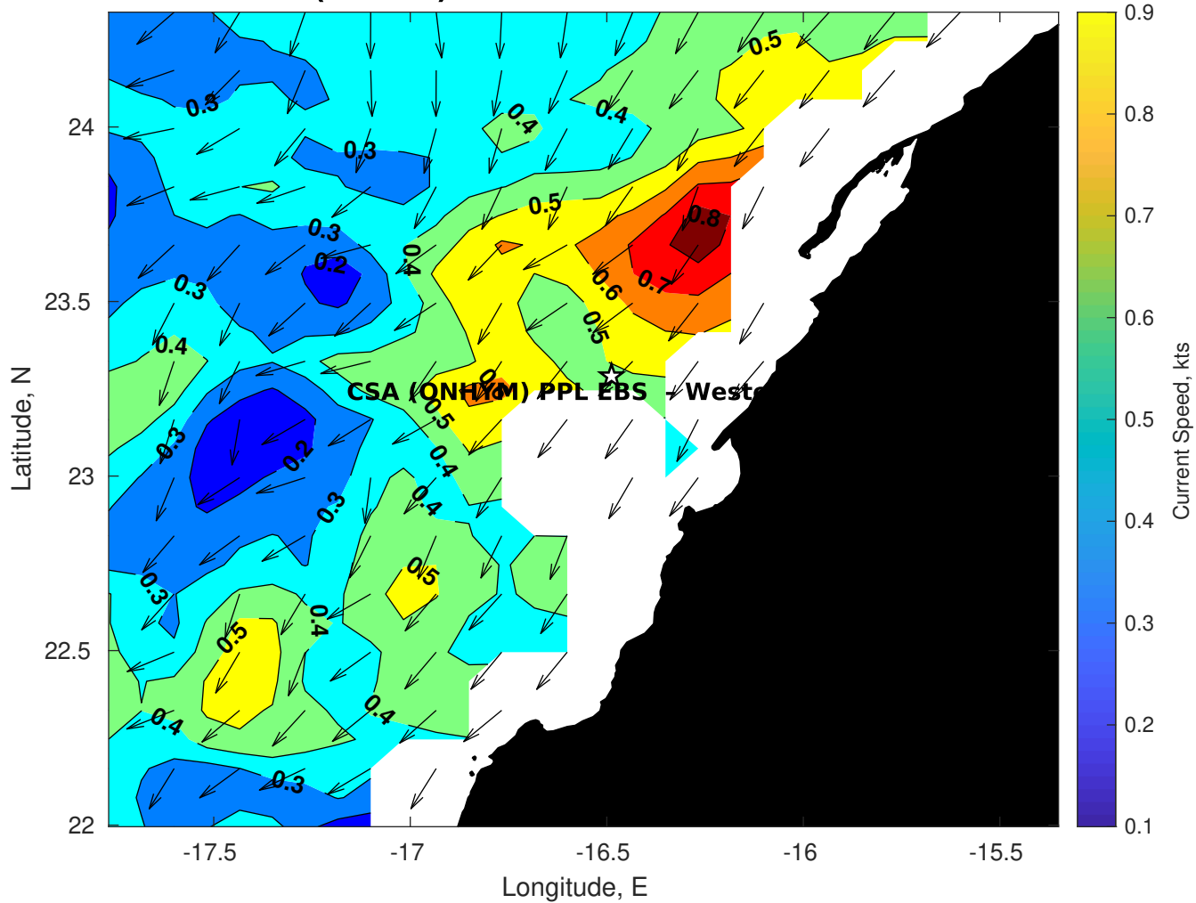
Surface Currents for CSA (ONHYM) PPL EBS - Western Sahara at 09-Nov-2025 00:00:00
