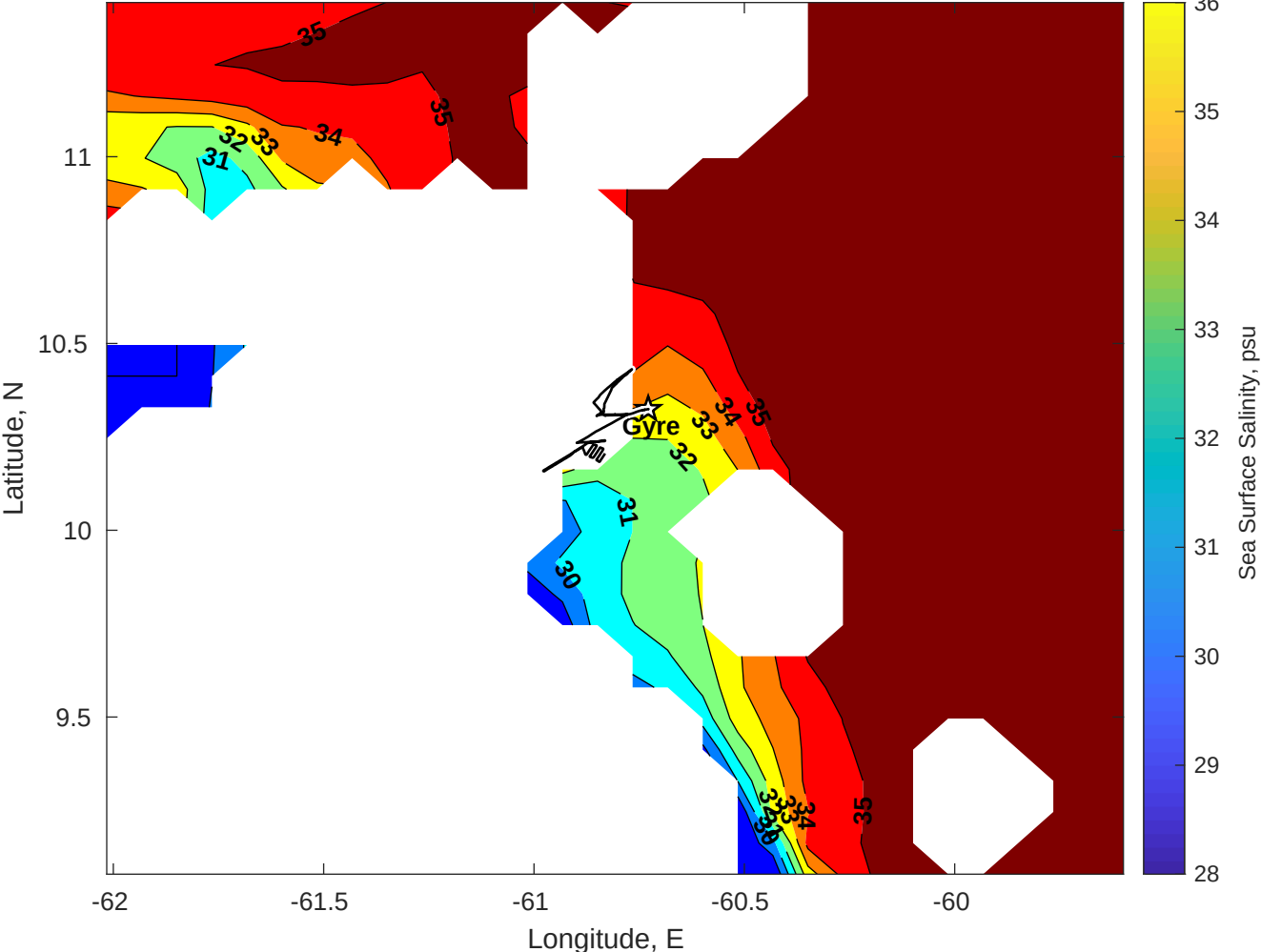
Surface Salinity for Gyre at 09-Nov-2025 00:00:00
