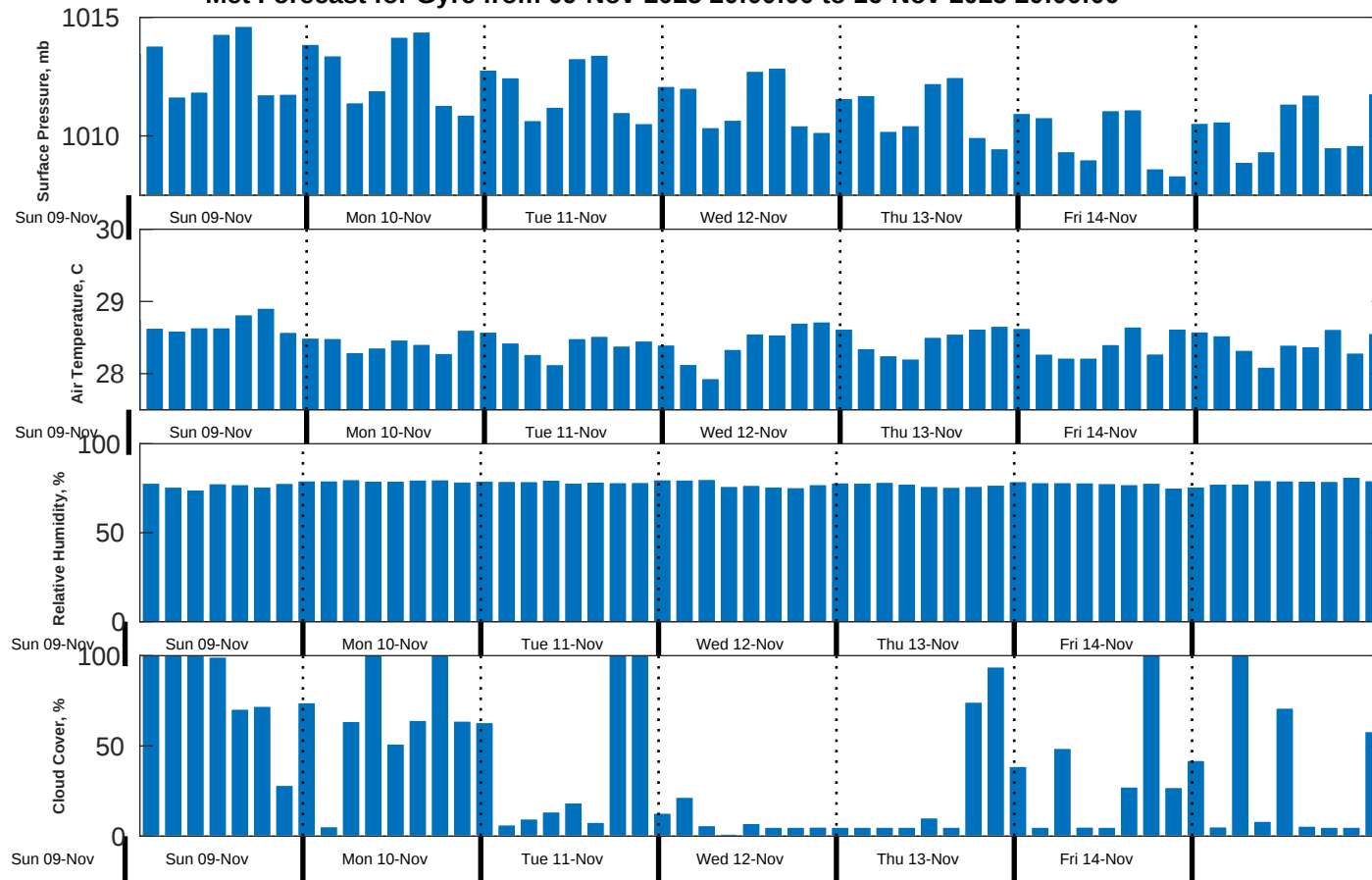
Met Forecast for Gyre from 09-Nov-2025 20:00:00 to 16-Nov-2025 20:00:00
