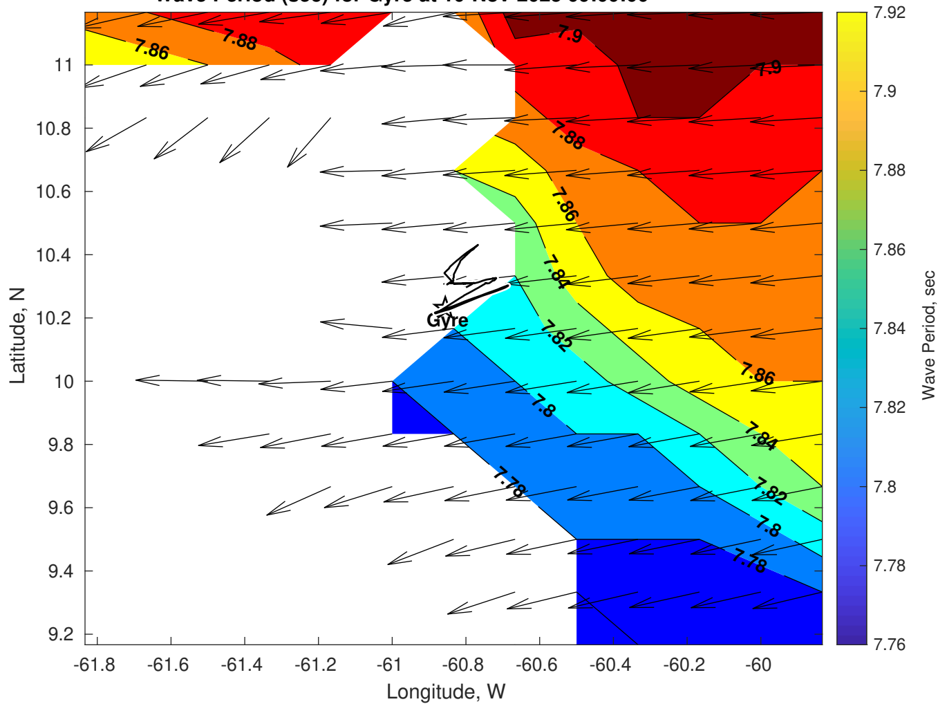
Wave Period (sec) for Gyre at 10-Nov-2025 09:00:00
