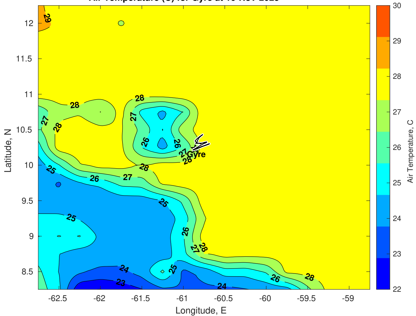
Air Temperature (C) for Gyre at 10-Nov-2025
