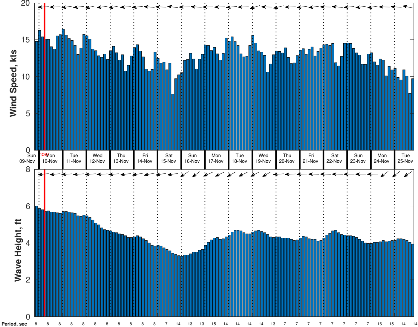
Wind & Wave Forecast for Gyre from 09-Nov-2025 20:00:00 to 25-Nov-2025 20:00:00
