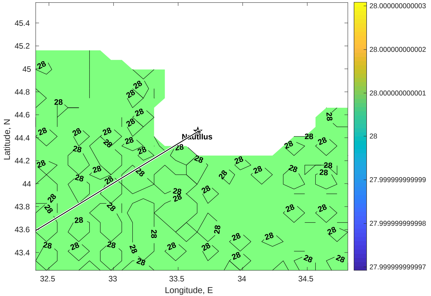
Surface Salinity for Nautilus at 09-Nov-2025 00:00:00
