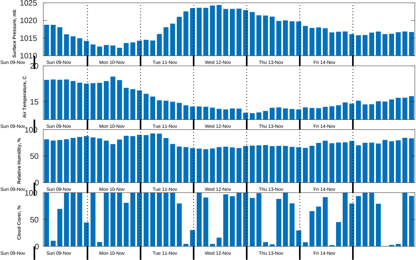
Met Forecast for Nautilus from 10-Nov-2025 00:00:00 to 17-Nov-2025 00:00:00
